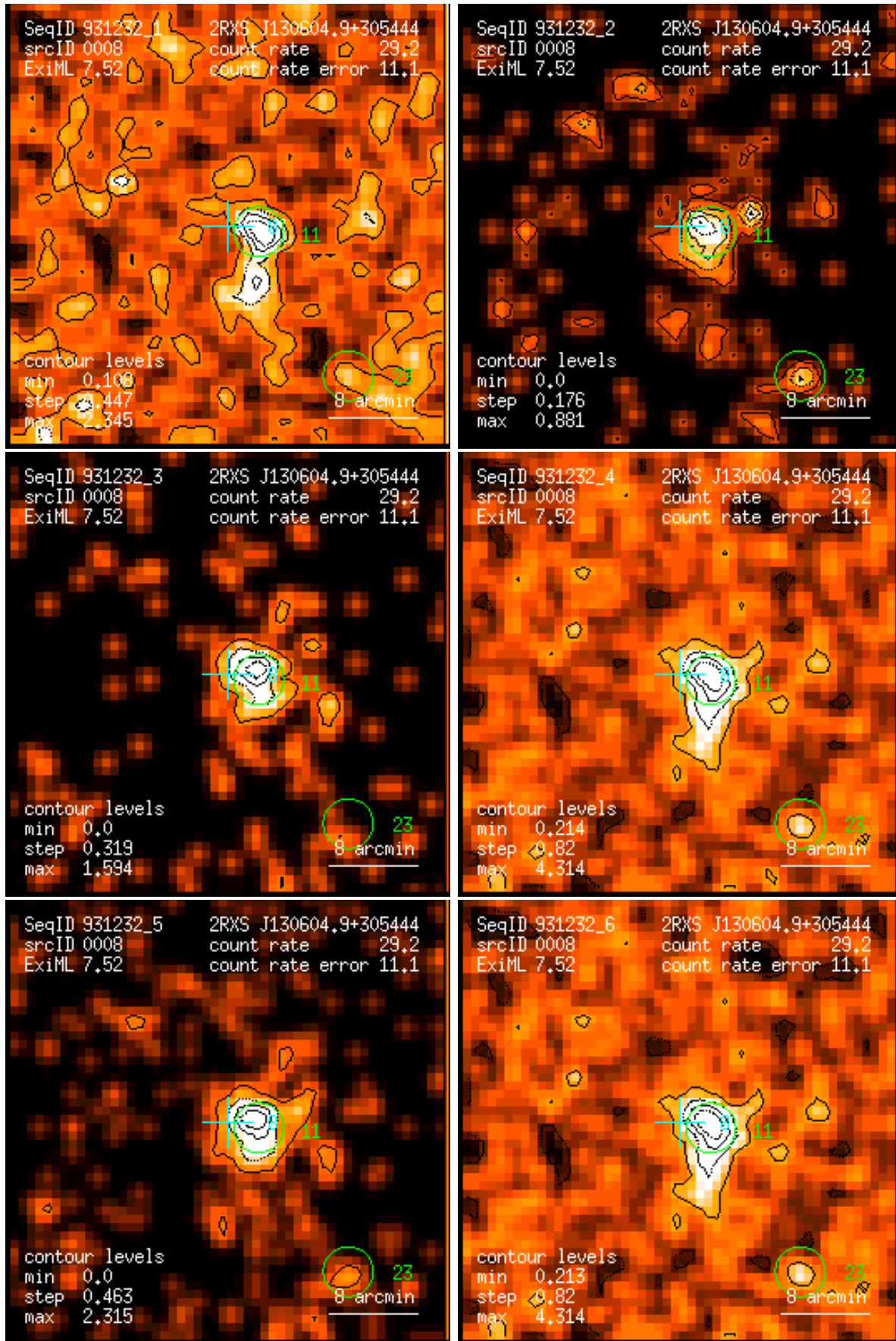
Figure 8: RASS 931232: detection 0008: band rate images, Gaussian filter: (1) PSPC channels 11 – 41, (2) 52 – 90, (3) 91 – 201, (4) 11 – 235, (5) 52 – 201, (6) 11 – 201. Broad band rates in counts/ks. Band rate contour levels in counts/ks/arcmin 2 .
