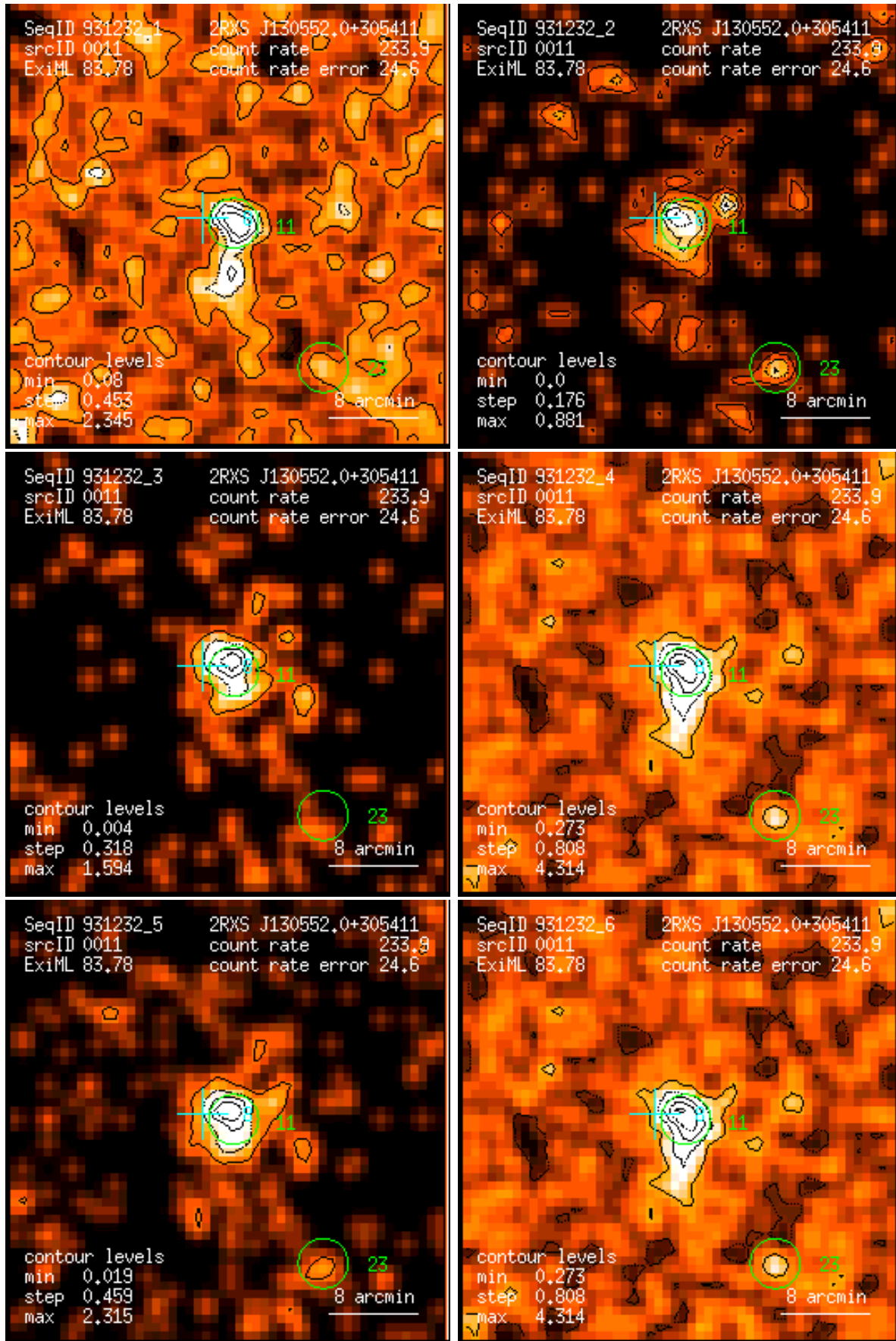
Figure 11: RASS 931232: detection 0011: band rate images, Gaussian filter: (1) PSPC channels 11 – 41, (2) 52 – 90, (3) 91 – 201, (4) 11 – 235, (5) 52 – 201, (6) 11 – 201. Broad band rates in counts/ks. Band rate contour levels in counts/ks/arcmin 2 .
