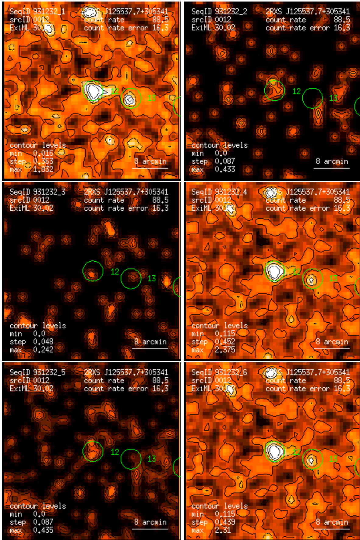
Figure 12: RASS 931232: detection 0012: band rate images, Gaussian filter: (1) PSPC channels 11 – 41, (2) 52 – 90, (3) 91 – 201, (4) 11 – 235, (5) 52 – 201, (6) 11 – 201. Broad band rates in counts/ks. Band rate contour levels in counts/ks/arcmin 2 .
