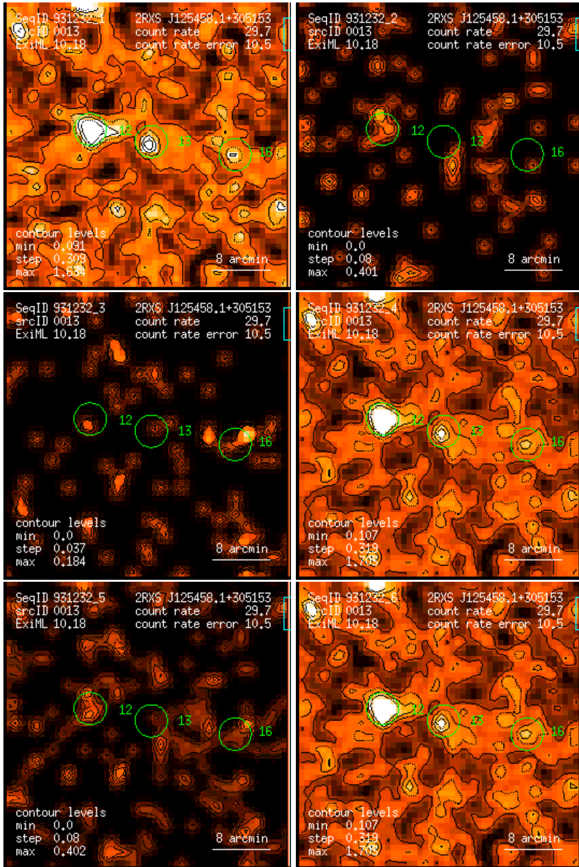
Figure 13: RASS 931232: detection 0013: band rate images, Gaussian filter: (1) PSPC channels 11 – 41, (2) 52 – 90, (3) 91 – 201, (4) 11 – 235, (5) 52 – 201, (6) 11 – 201. Broad band rates in counts/ks. Band rate contour levels in counts/ks/arcmin 2 .
