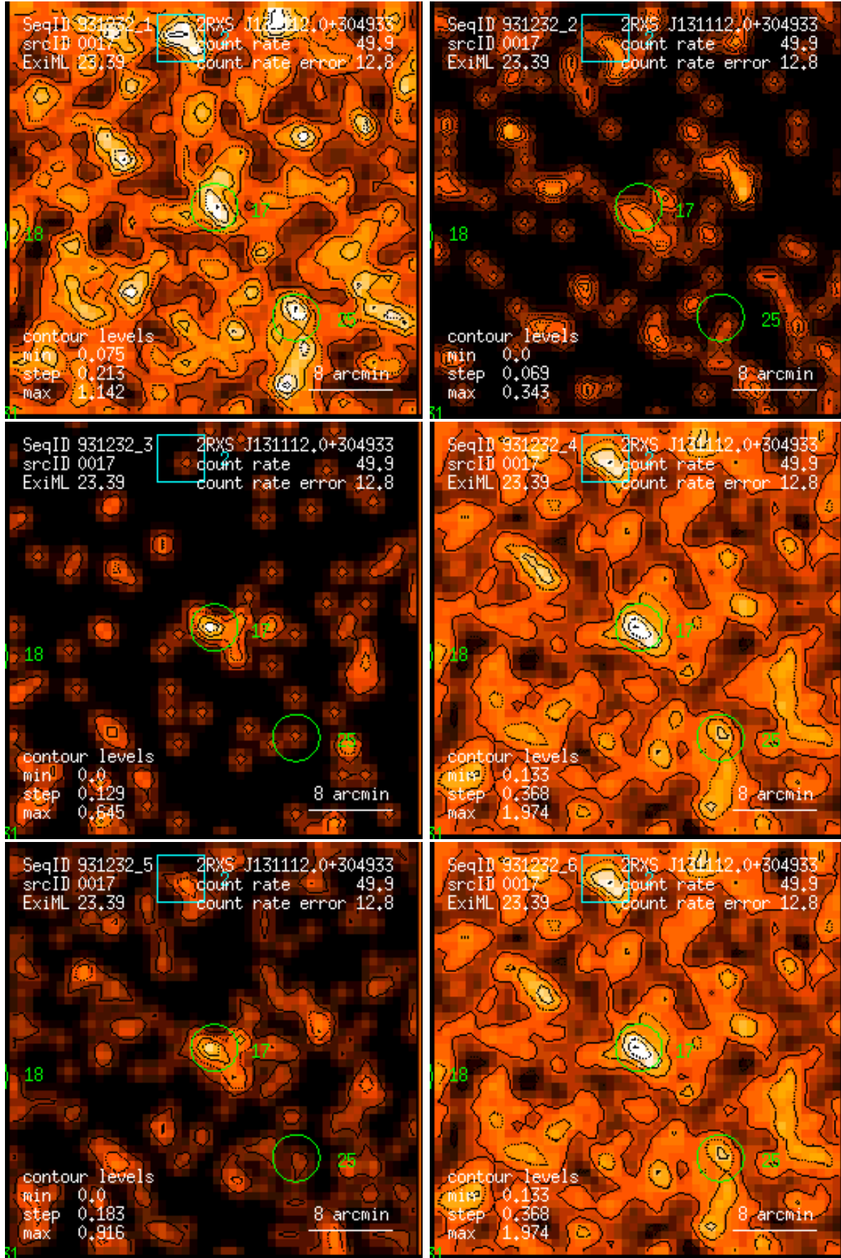
Figure 17: RASS 931232: detection 0017: band rate images, Gaussian filter: (1) PSPC channels 11 – 41, (2) 52 – 90, (3) 91 – 201, (4) 11 – 235, (5) 52 – 201, (6) 11 – 201. Broad band rates in counts/ks. Band rate contour levels in counts/ks/arcmin 2 .
