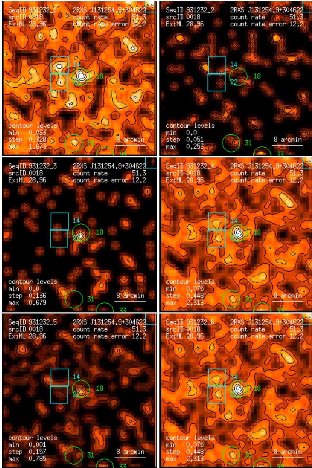
Figure 18: RASS 931232: detection 0018: band rate images, Gaussian filter: (1) PSPC channels 11 – 41, (2) 52 – 90, (3) 91 – 201, (4) 11 – 235, (5) 52 – 201, (6) 11 – 201. Broad band rates in counts/ks. Band rate contour levels in counts/ks/arcmin 2 .
