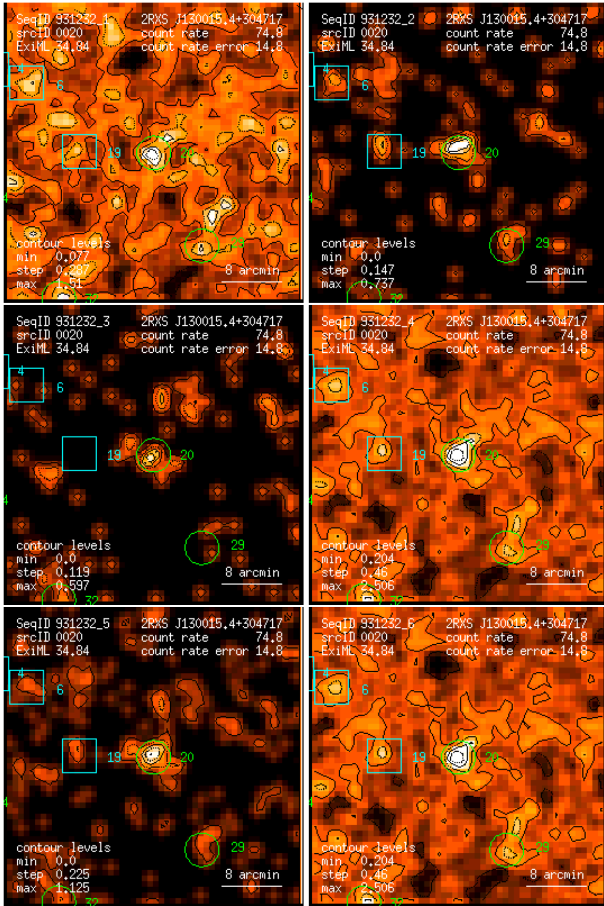
Figure 20: RASS 931232: detection 0020: band rate images, Gaussian filter: (1) PSPC channels 11 – 41, (2) 52 – 90, (3) 91 – 201, (4) 11 – 235, (5) 52 – 201, (6) 11 – 201. Broad band rates in counts/ks. Band rate contour levels in counts/ks/arcmin 2 .
