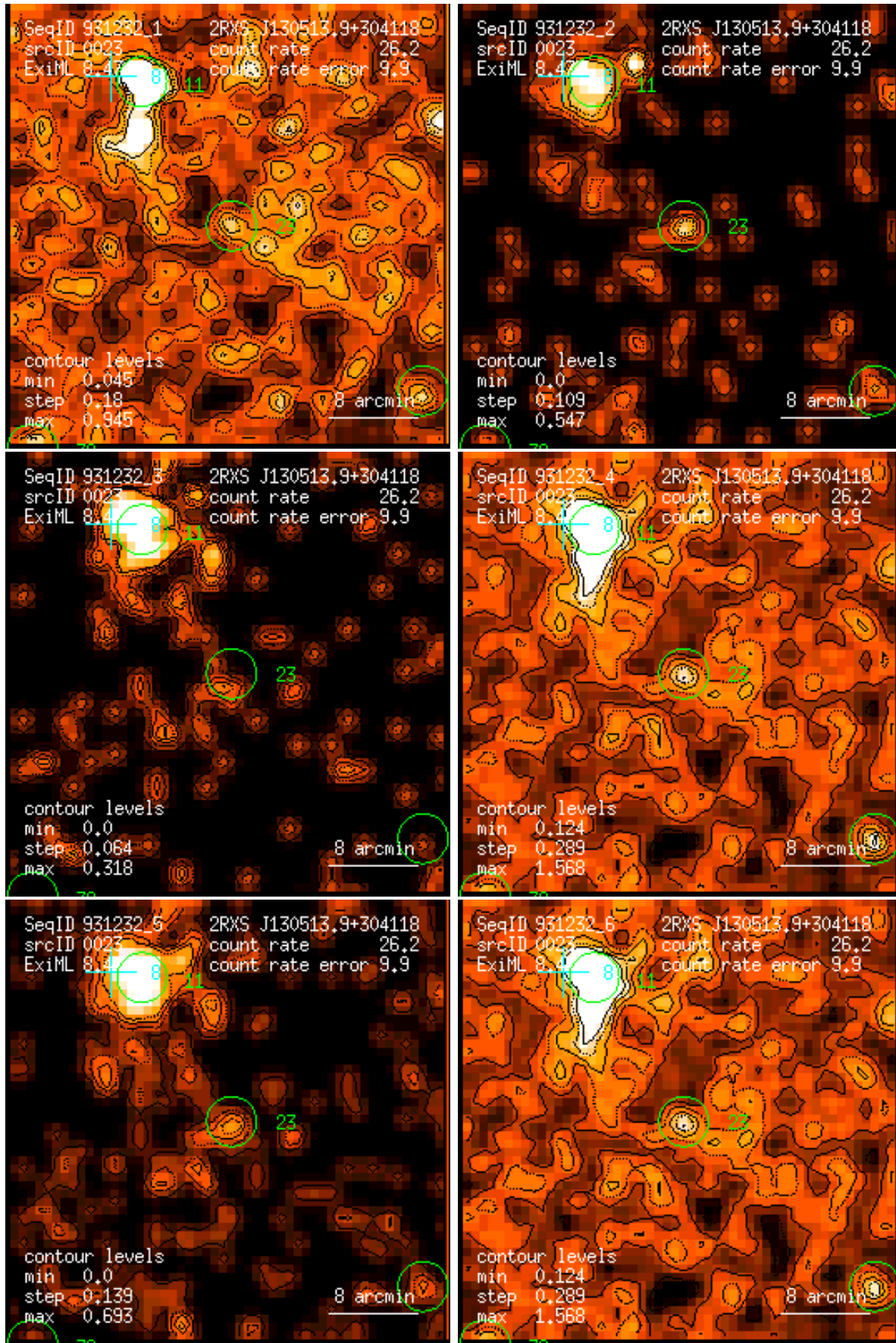
Figure 23: RASS 931232: detection 0023: band rate images, Gaussian filter: (1) PSPC channels 11 – 41, (2) 52 – 90, (3) 91 – 201, (4) 11 – 235, (5) 52 – 201, (6) 11 – 201. Broad band rates in counts/ks. Band rate contour levels in counts/ks/arcmin 2 .
