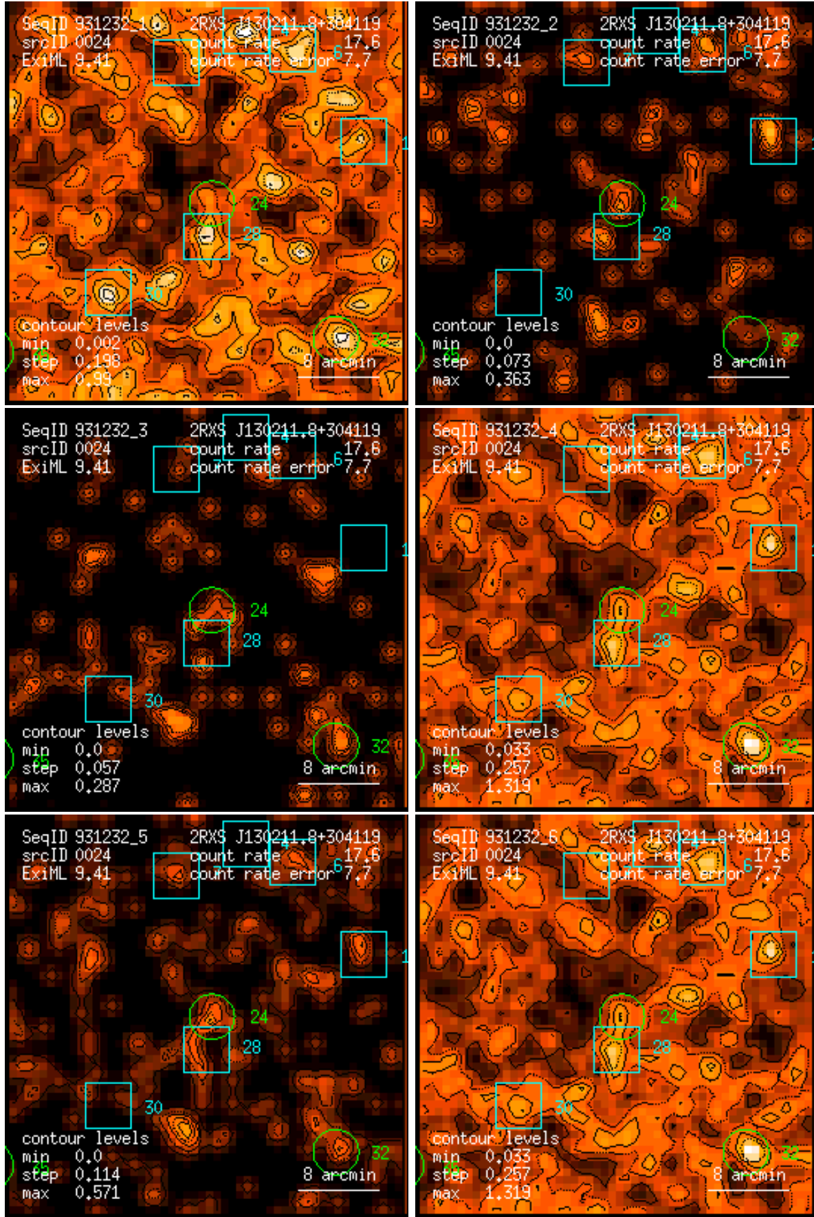
Figure 24: RASS 931232: detection 0024: band rate images, Gaussian filter: (1) PSPC channels 11 – 41, (2) 52 – 90, (3) 91 – 201, (4) 11 – 235, (5) 52 – 201, (6) 11 – 201. Broad band rates in counts/ks. Band rate contour levels in counts/ks/arcmin 2 .
