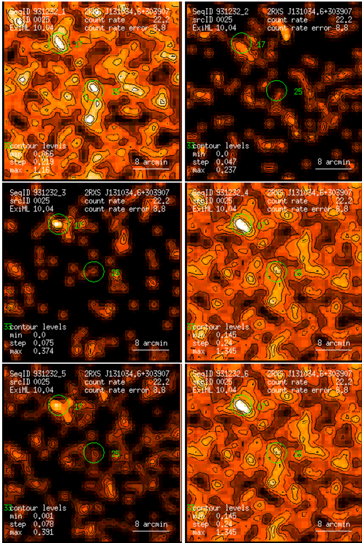
Figure 25: RASS 931232: detection 0025: band rate images, Gaussian filter: (1) PSPC channels 11 – 41, (2) 52 – 90, (3) 91 – 201, (4) 11 – 235, (5) 52 – 201, (6) 11 – 201. Broad band rates in counts/ks. Band rate contour levels in counts/ks/arcmin 2 .
