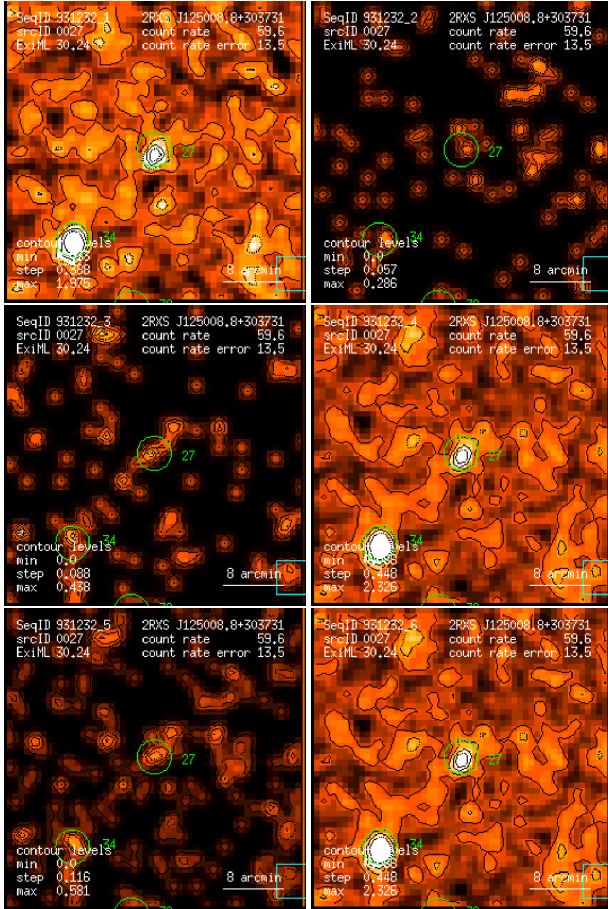
Figure 27: RASS 931232: detection 0027: band rate images, Gaussian filter: (1) PSPC channels 11 – 41, (2) 52 – 90, (3) 91 – 201, (4) 11 – 235, (5) 52 – 201, (6) 11 – 201. Broad band rates in counts/ks. Band rate contour levels in counts/ks/arcmin 2 .
