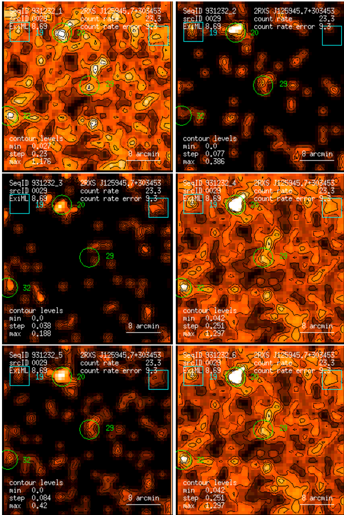
Figure 29: RASS 931232: detection 0029: band rate images, Gaussian filter: (1) PSPC channels 11 – 41, (2) 52 – 90, (3) 91 – 201, (4) 11 – 235, (5) 52 – 201, (6) 11 – 201. Broad band rates in counts/ks. Band rate contour levels in counts/ks/arcmin 2 .
