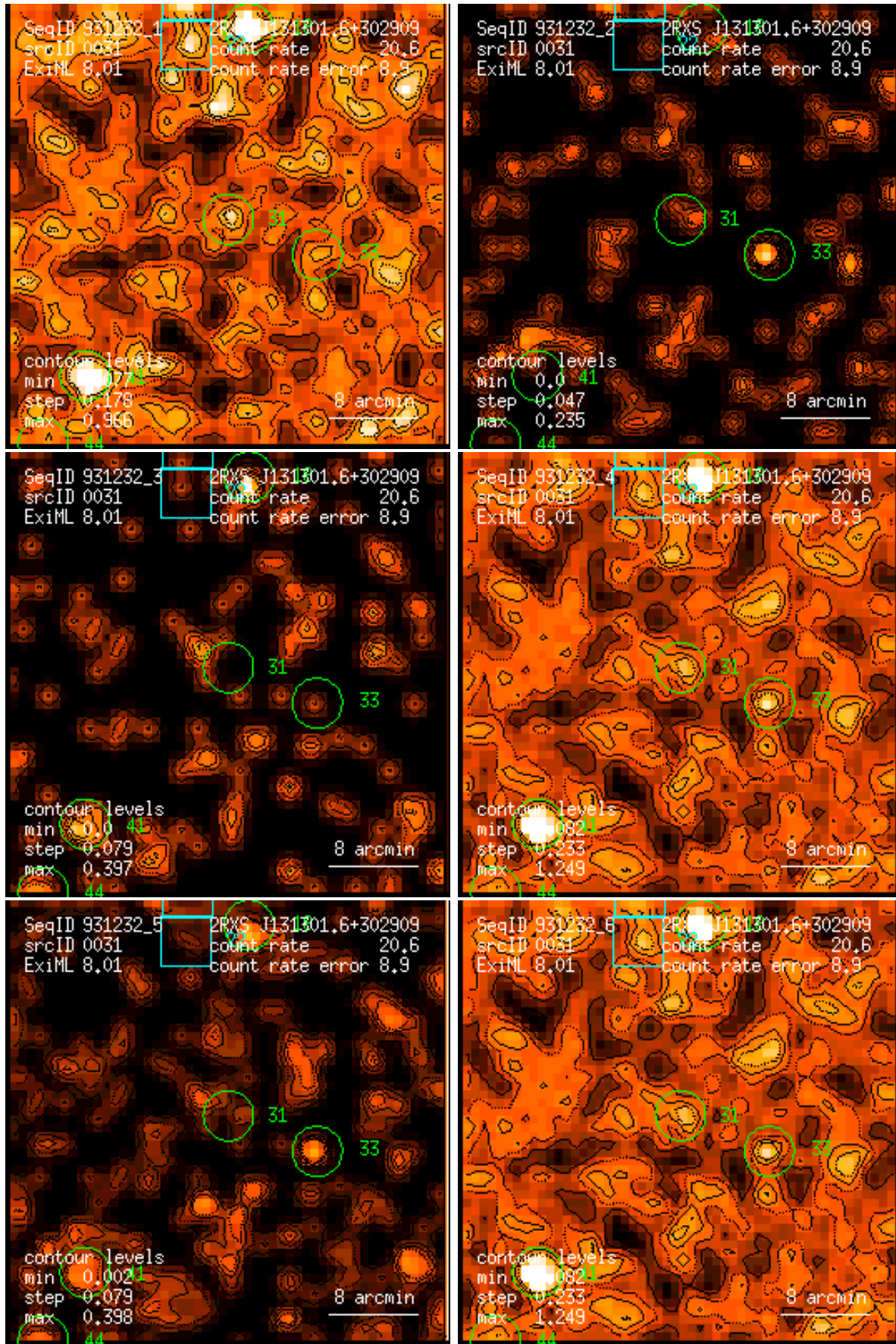
Figure 31: RASS 931232: detection 0031: band rate images, Gaussian filter: (1) PSPC channels 11 – 41, (2) 52 – 90, (3) 91 – 201, (4) 11 – 235, (5) 52 – 201, (6) 11 – 201. Broad band rates in counts/ks. Band rate contour levels in counts/ks/arcmin 2 .
