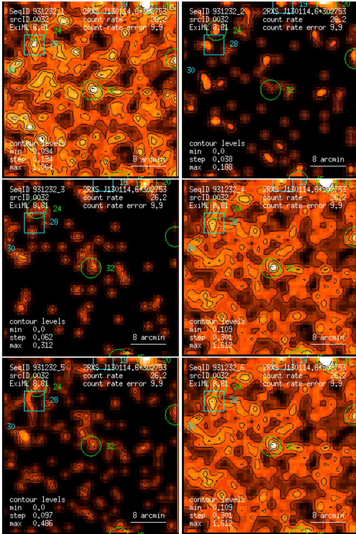
Figure 32: RASS 931232: detection 0032: band rate images, Gaussian filter: (1) PSPC channels 11 – 41, (2) 52 – 90, (3) 91 – 201, (4) 11 – 235, (5) 52 – 201, (6) 11 – 201. Broad band rates in counts/ks. Band rate contour levels in counts/ks/arcmin 2 .
