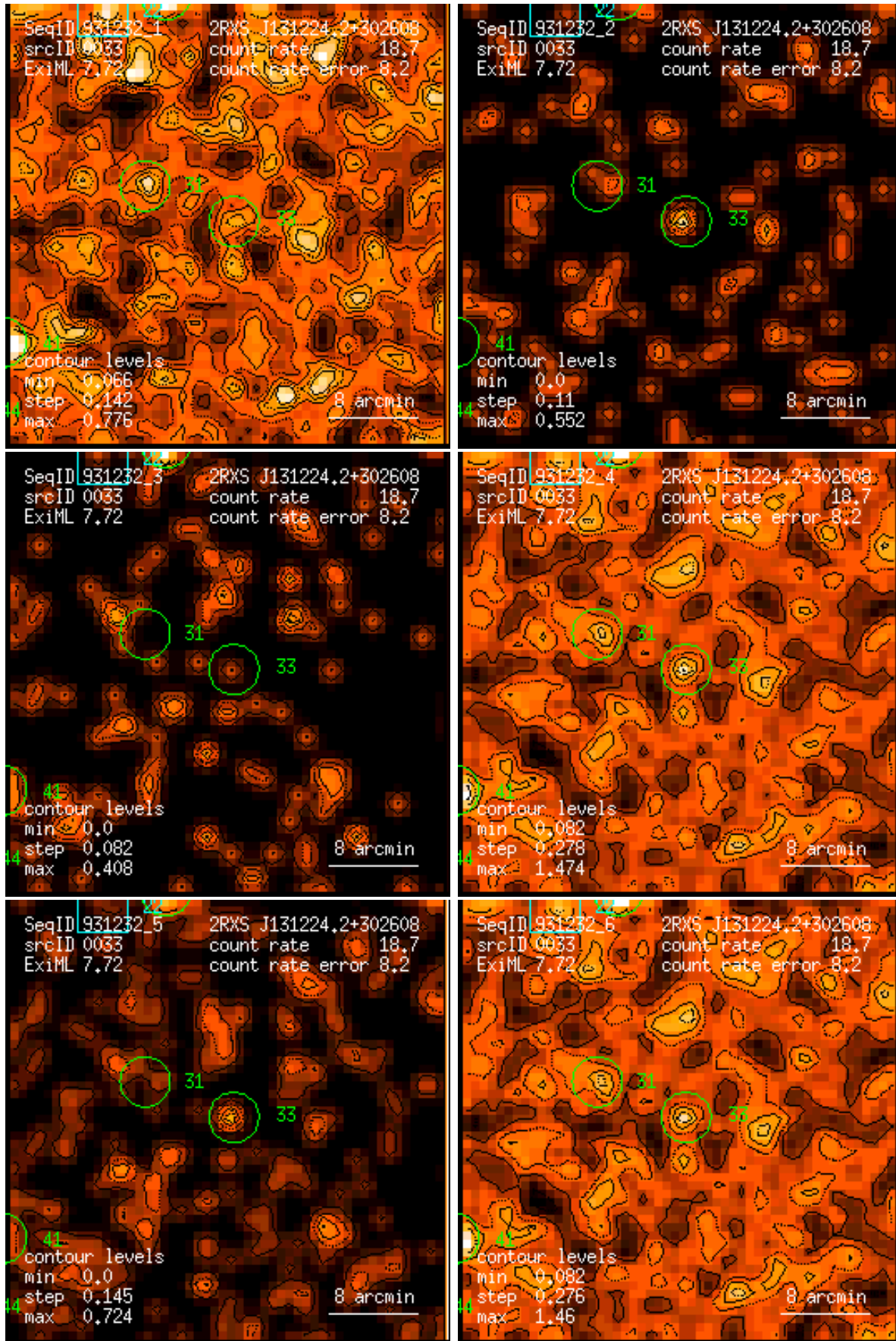
Figure 33: RASS 931232: detection 0033: band rate images, Gaussian filter: (1) PSPC channels 11 – 41, (2) 52 – 90, (3) 91 – 201, (4) 11 – 235, (5) 52 – 201, (6) 11 – 201. Broad band rates in counts/ks. Band rate contour levels in counts/ks/arcmin 2 .
