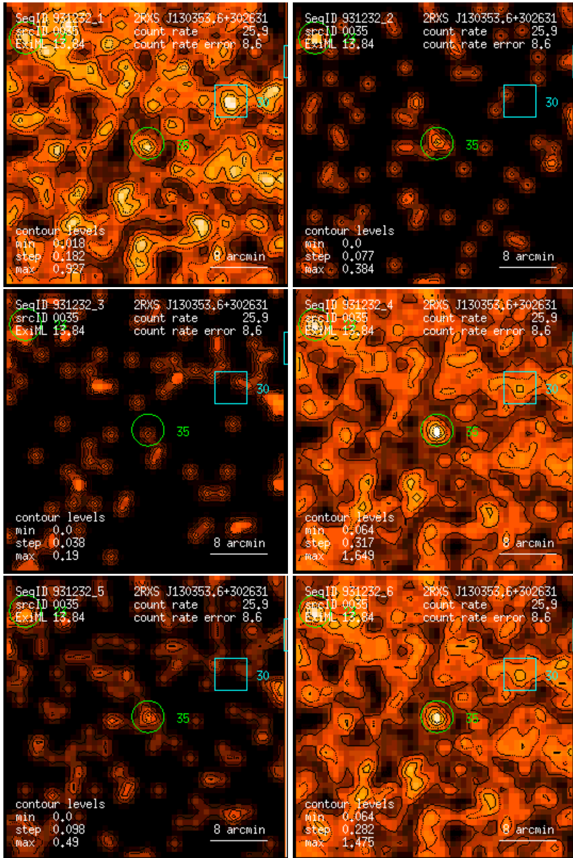
Figure 35: RASS 931232: detection 0035: band rate images, Gaussian filter: (1) PSPC channels 11 – 41, (2) 52 – 90, (3) 91 – 201, (4) 11 – 235, (5) 52 – 201, (6) 11 – 201. Broad band rates in counts/ks. Band rate contour levels in counts/ks/arcmin 2 .
