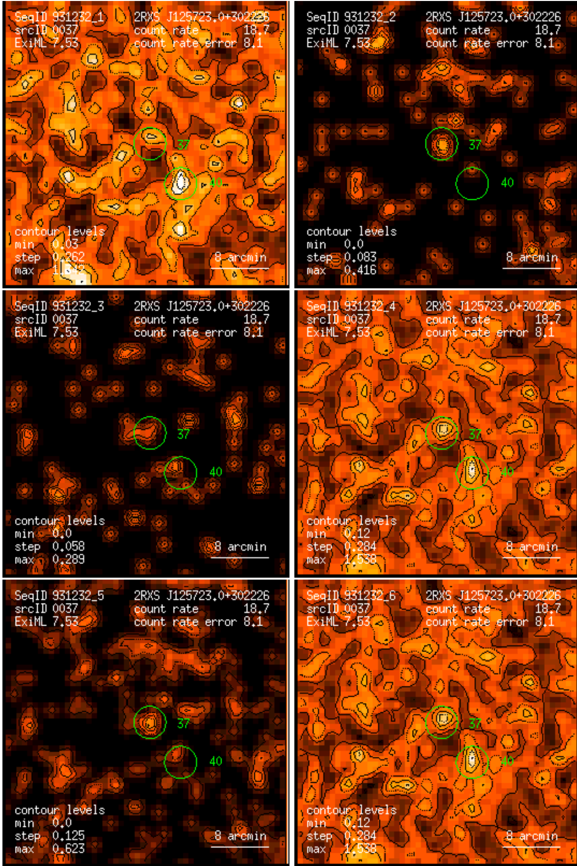
Figure 37: RASS 931232: detection 0037: band rate images, Gaussian filter: (1) PSPC channels 11 – 41, (2) 52 – 90, (3) 91 – 201, (4) 11 – 235, (5) 52 – 201, (6) 11 – 201. Broad band rates in counts/ks. Band rate contour levels in counts/ks/arcmin 2 .
