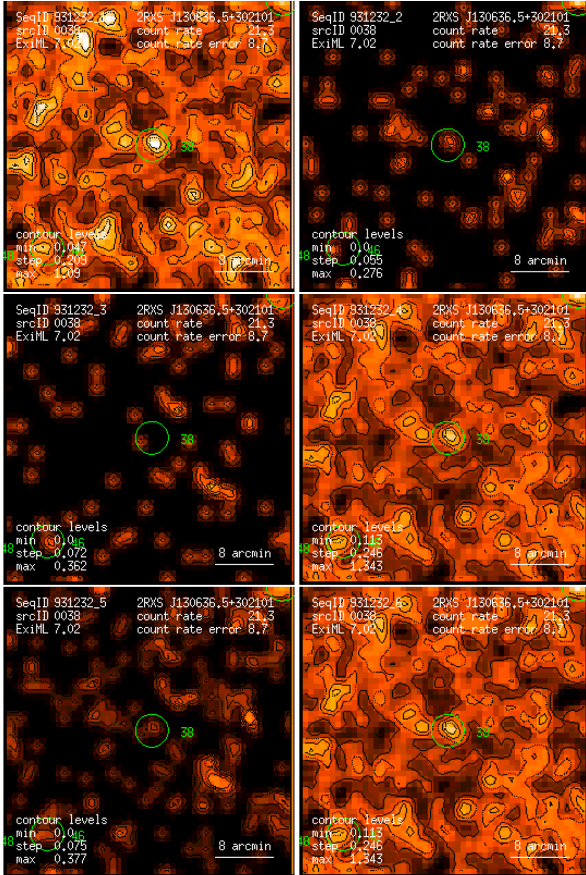
Figure 38: RASS 931232: detection 0038: band rate images, Gaussian filter: (1) PSPC channels 11 – 41, (2) 52 – 90, (3) 91 – 201, (4) 11 – 235, (5) 52 – 201, (6) 11 – 201. Broad band rates in counts/ks. Band rate contour levels in counts/ks/arcmin 2 .
