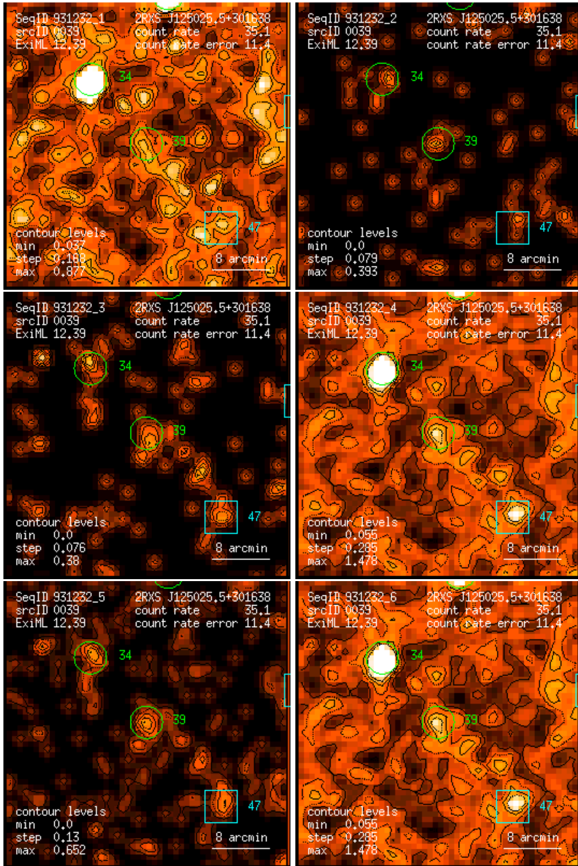
Figure 39: RASS 931232: detection 0039: band rate images, Gaussian filter: (1) PSPC channels 11 – 41, (2) 52 – 90, (3) 91 – 201, (4) 11 – 235, (5) 52 – 201, (6) 11 – 201. Broad band rates in counts/ks. Band rate contour levels in counts/ks/arcmin 2 .
