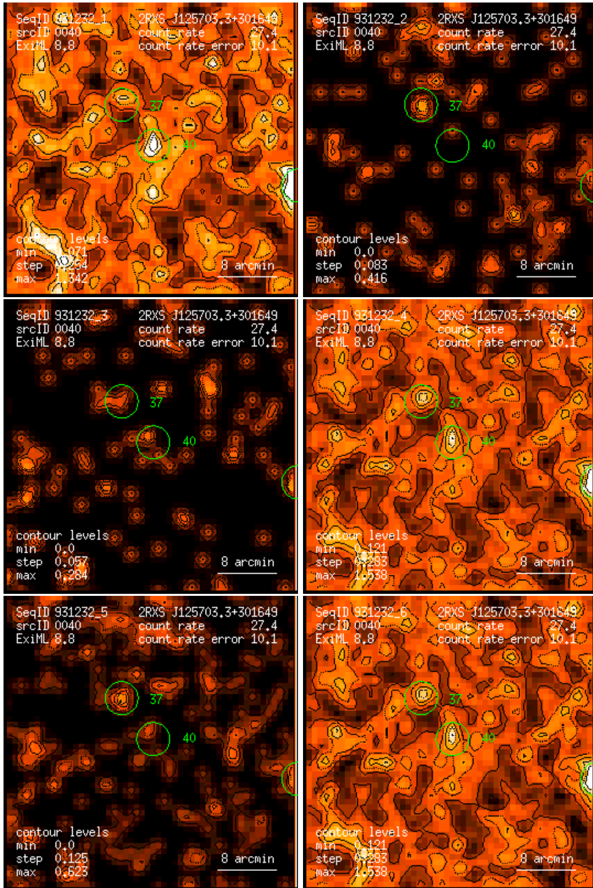
Figure 40: RASS 931232: detection 0040: band rate images, Gaussian filter: (1) PSPC channels 11 – 41, (2) 52 – 90, (3) 91 – 201, (4) 11 – 235, (5) 52 – 201, (6) 11 – 201. Broad band rates in counts/ks. Band rate contour levels in counts/ks/arcmin 2 .
