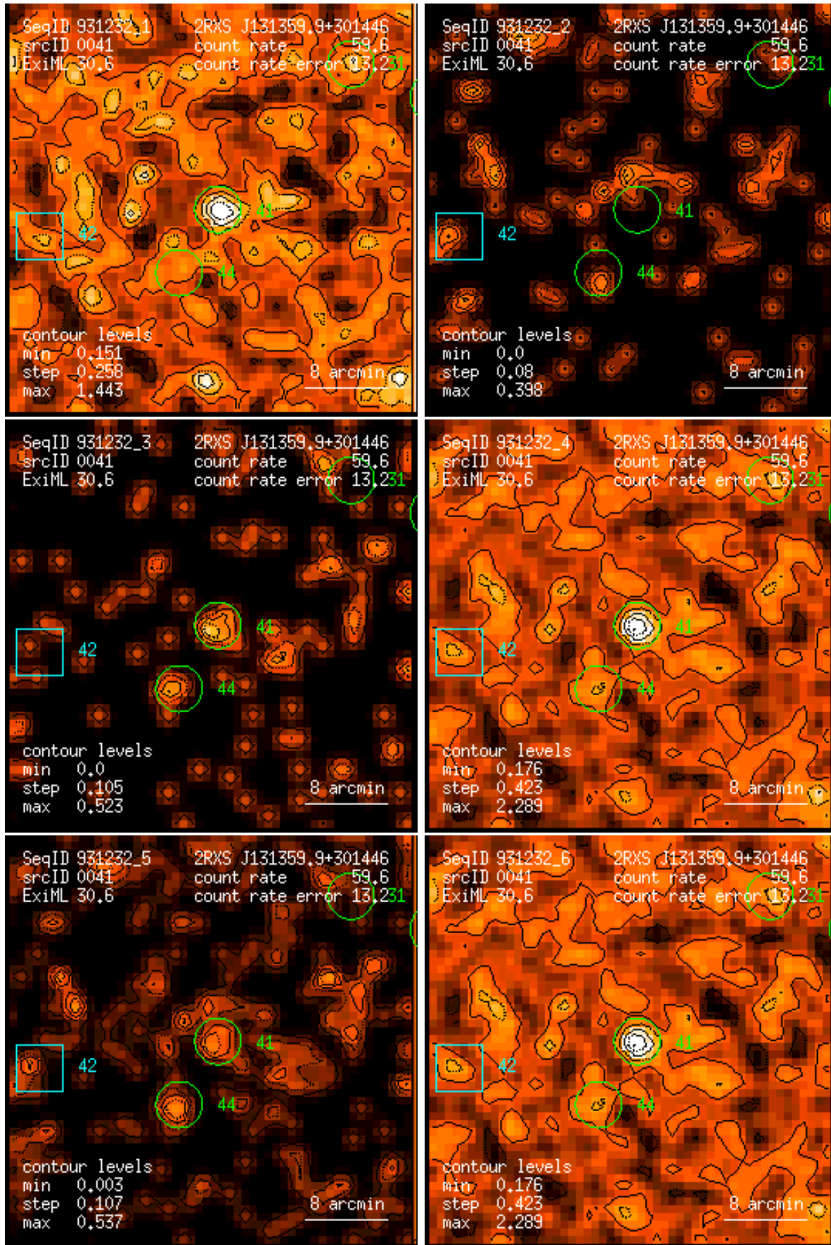
Figure 41: RASS 931232: detection 0041: band rate images, Gaussian filter: (1) PSPC channels 11 – 41, (2) 52 – 90, (3) 91 – 201, (4) 11 – 235, (5) 52 – 201, (6) 11 – 201. Broad band rates in counts/ks. Band rate contour levels in counts/ks/arcmin 2 .
