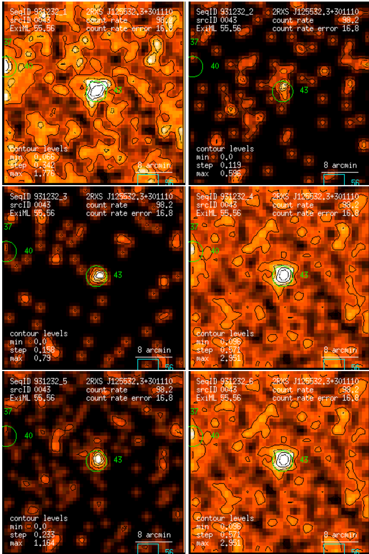
Figure 43: RASS 931232: detection 0043: band rate images, Gaussian filter: (1) PSPC channels 11 – 41, (2) 52 – 90, (3) 91 – 201, (4) 11 – 235, (5) 52 – 201, (6) 11 – 201. Broad band rates in counts/ks. Band rate contour levels in counts/ks/arcmin 2 .
