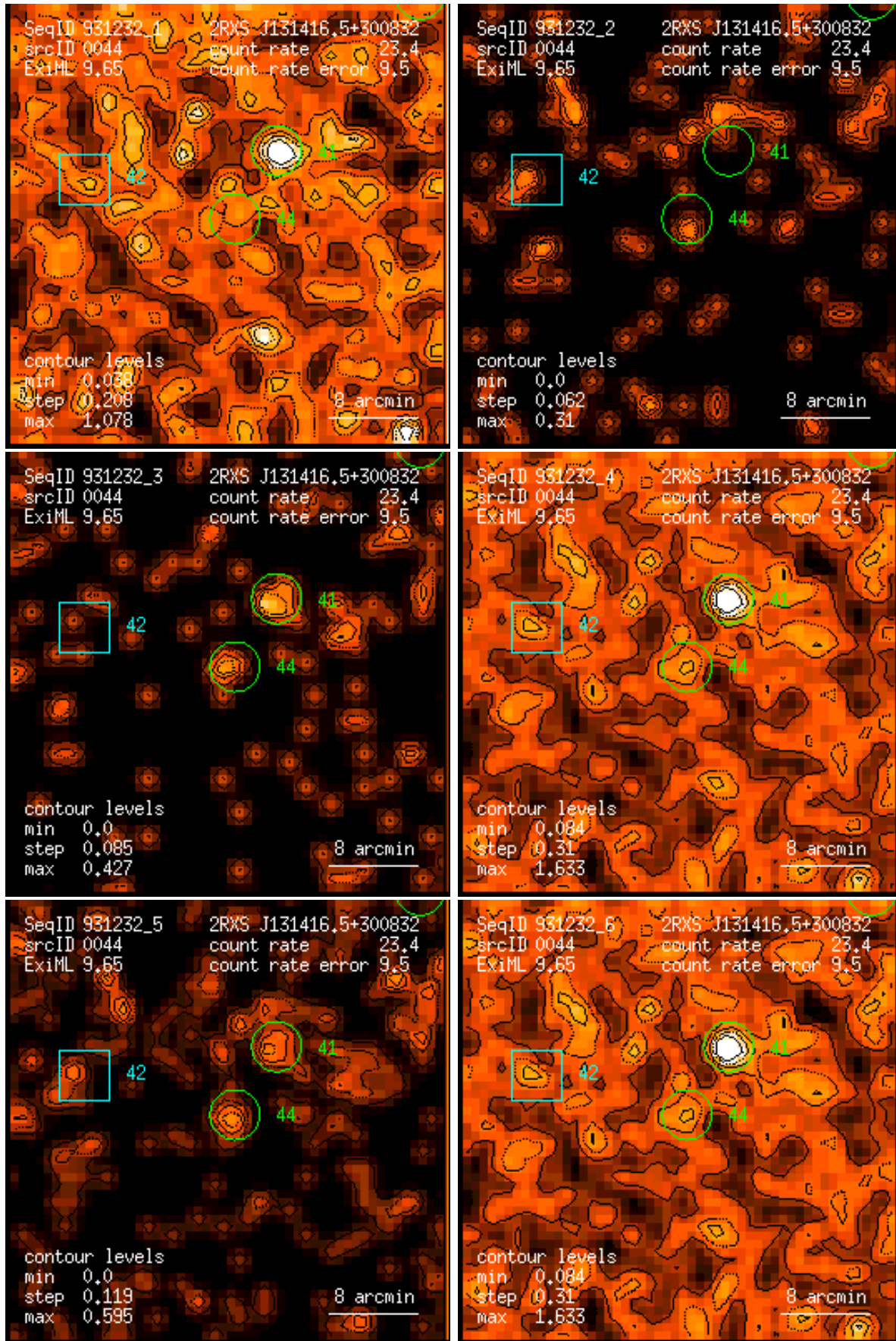
Figure 44: RASS 931232: detection 0044: band rate images, Gaussian filter: (1) PSPC channels 11 – 41, (2) 52 – 90, (3) 91 – 201, (4) 11 – 235, (5) 52 – 201, (6) 11 – 201. Broad band rates in counts/ks. Band rate contour levels in counts/ks/arcmin 2 .
