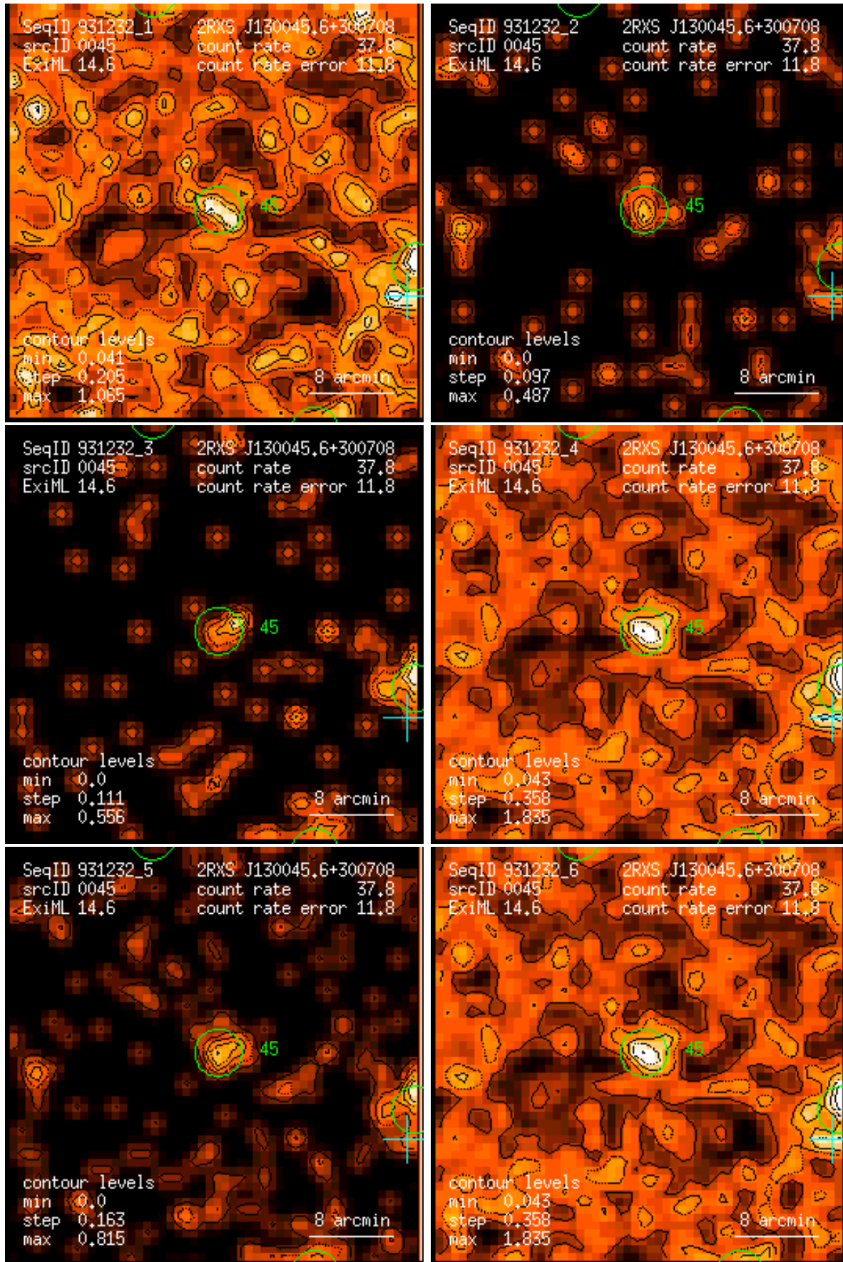
Figure 45: RASS 931232: detection 0045: band rate images, Gaussian filter: (1) PSPC channels 11 – 41, (2) 52 – 90, (3) 91 – 201, (4) 11 – 235, (5) 52 – 201, (6) 11 – 201. Broad band rates in counts/ks. Band rate contour levels in counts/ks/arcmin 2 .
