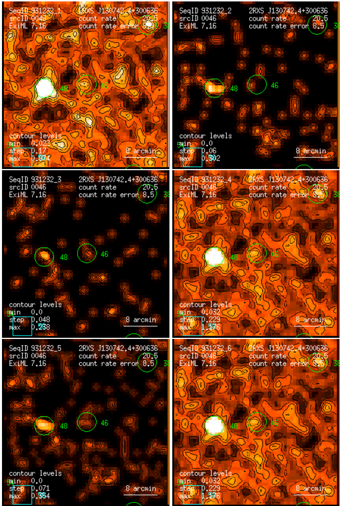
Figure 46: RASS 931232: detection 0046: band rate images, Gaussian filter: (1) PSPC channels 11 – 41, (2) 52 – 90, (3) 91 – 201, (4) 11 – 235, (5) 52 – 201, (6) 11 – 201. Broad band rates in counts/ks. Band rate contour levels in counts/ks/arcmin 2 .
