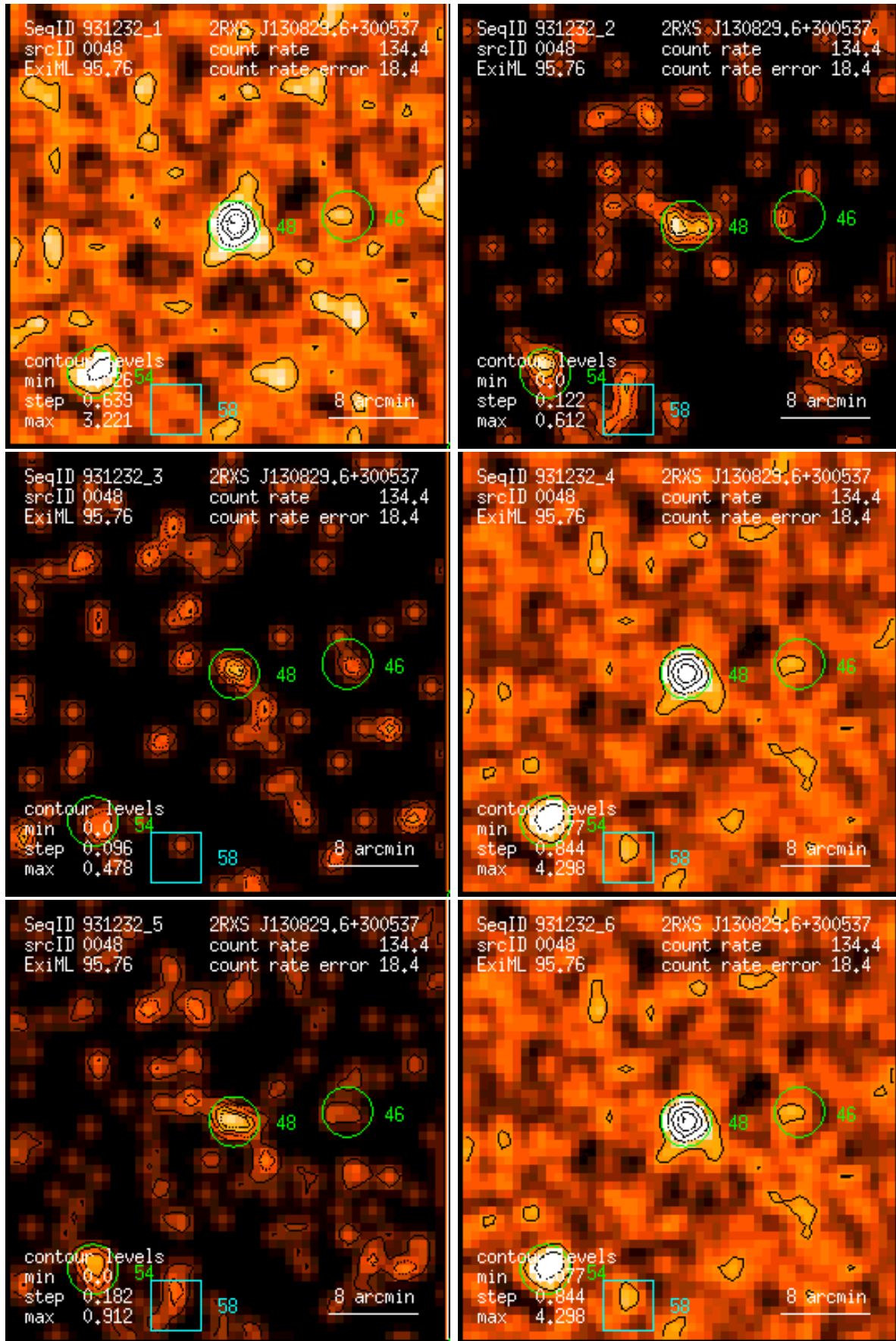
Figure 48: RASS 931232: detection 0048: band rate images, Gaussian filter: (1) PSPC channels 11 – 41, (2) 52 – 90, (3) 91 – 201, (4) 11 – 235, (5) 52 – 201, (6) 11 – 201. Broad band rates in counts/ks. Band rate contour levels in counts/ks/arcmin 2 .
