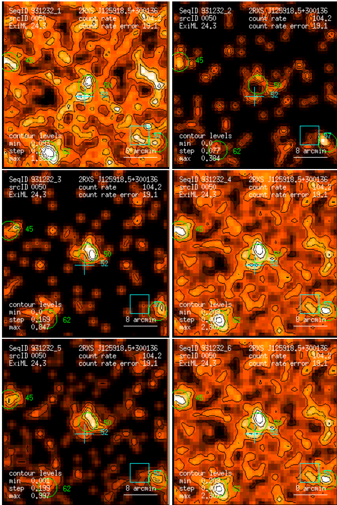
Figure 50: RASS 931232: detection 0050: band rate images, Gaussian filter: (1) PSPC channels 11 – 41, (2) 52 – 90, (3) 91 – 201, (4) 11 – 235, (5) 52 – 201, (6) 11 – 201. Broad band rates in counts/ks. Band rate contour levels in counts/ks/arcmin 2 .
