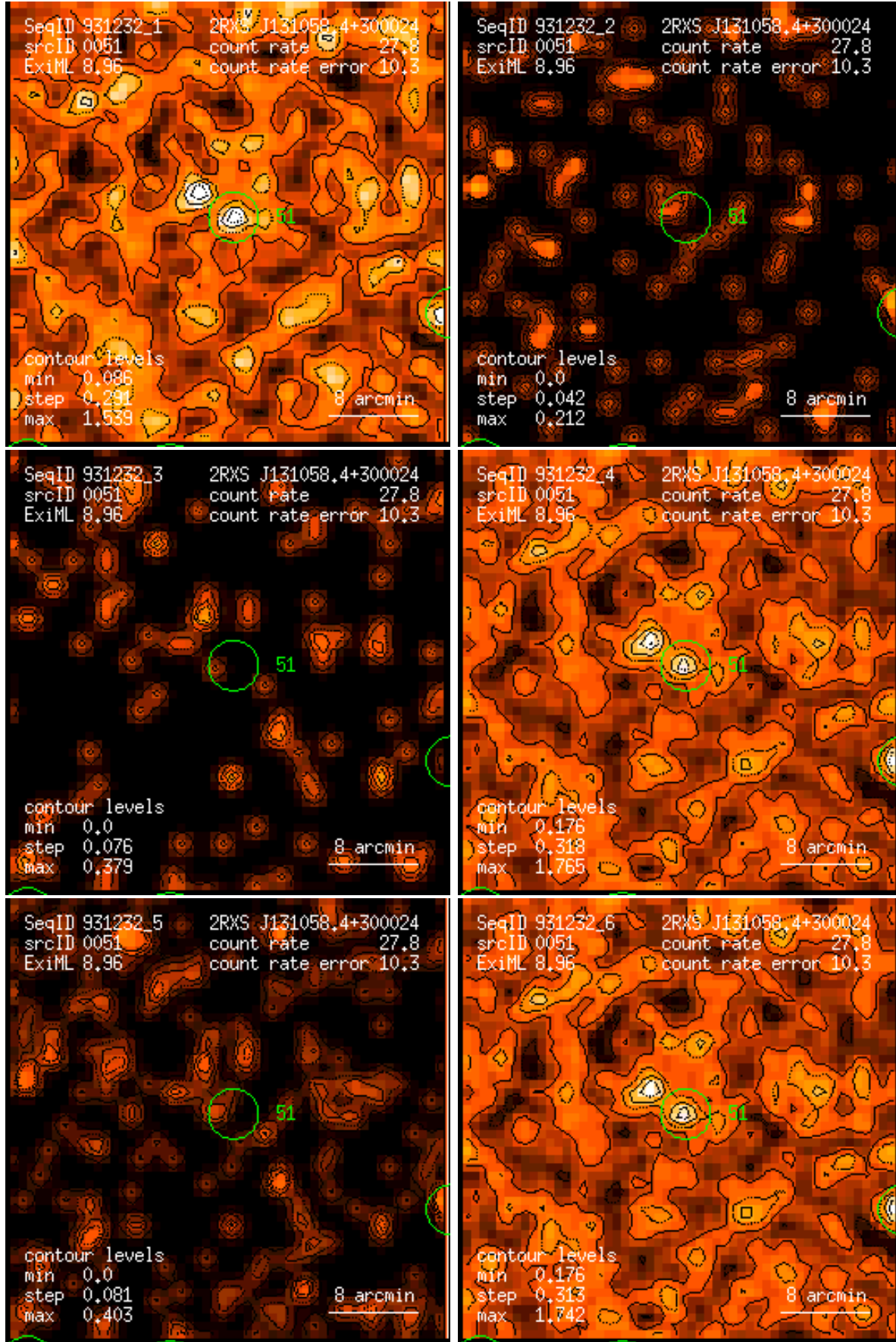
Figure 51: RASS 931232: detection 0051: band rate images, Gaussian filter: (1) PSPC channels 11 – 41, (2) 52 – 90, (3) 91 – 201, (4) 11 – 235, (5) 52 – 201, (6) 11 – 201. Broad band rates in counts/ks. Band rate contour levels in counts/ks/arcmin 2 .
