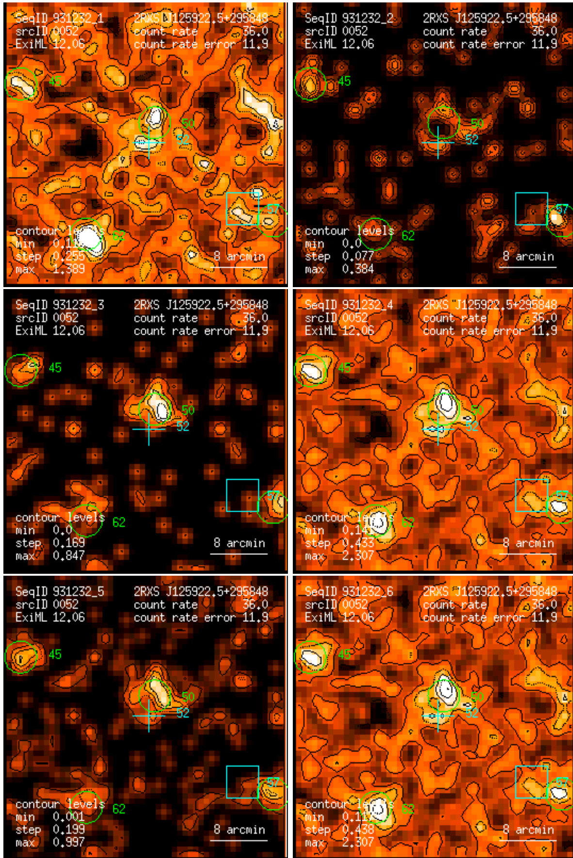
Figure 52: RASS 931232: detection 0052: band rate images, Gaussian filter: (1) PSPC channels 11 – 41, (2) 52 – 90, (3) 91 – 201, (4) 11 – 235, (5) 52 – 201, (6) 11 – 201. Broad band rates in counts/ks. Band rate contour levels in counts/ks/arcmin 2 .
