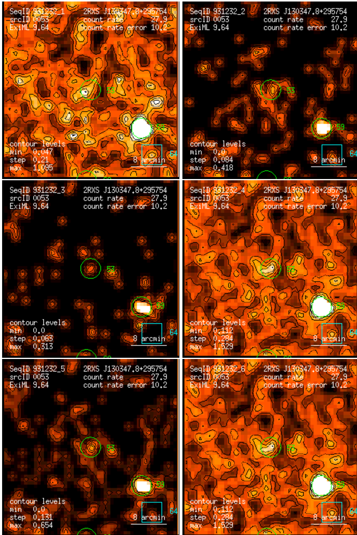
Figure 53: RASS 931232: detection 0053: band rate images, Gaussian filter: (1) PSPC channels 11 – 41, (2) 52 – 90, (3) 91 – 201, (4) 11 – 235, (5) 52 – 201, (6) 11 – 201. Broad band rates in counts/ks. Band rate contour levels in counts/ks/arcmin 2 .
