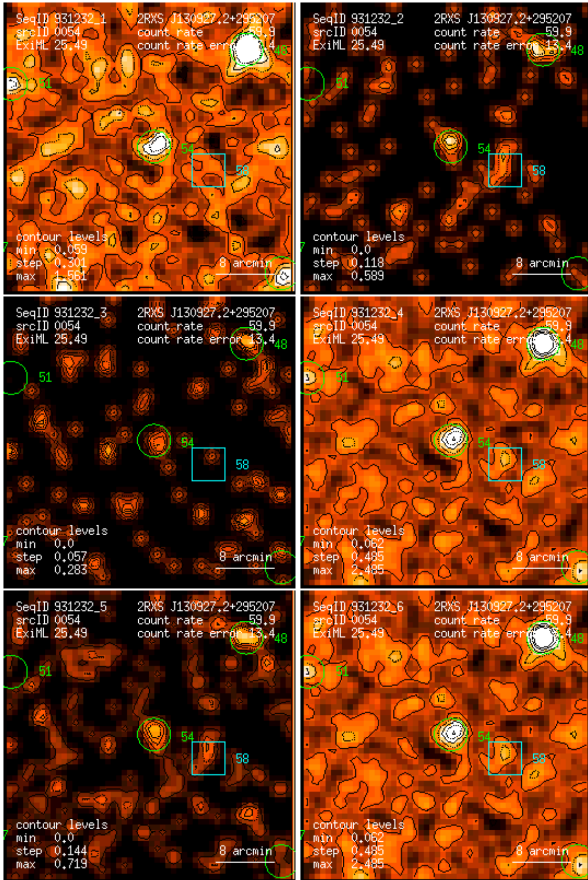
Figure 54: RASS 931232: detection 0054: band rate images, Gaussian filter: (1) PSPC channels 11 – 41, (2) 52 – 90, (3) 91 – 201, (4) 11 – 235, (5) 52 – 201, (6) 11 – 201. Broad band rates in counts/ks. Band rate contour levels in counts/ks/arcmin 2 .
