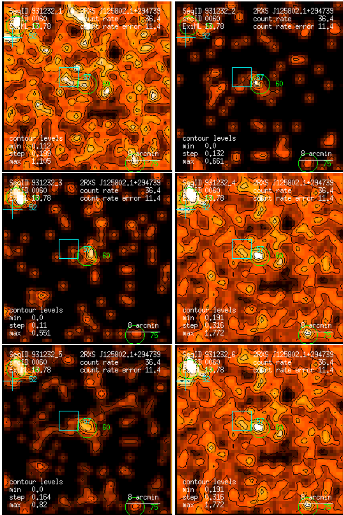
Figure 60: RASS 931232: detection 0060: band rate images, Gaussian filter: (1) PSPC channels 11 – 41, (2) 52 – 90, (3) 91 – 201, (4) 11 – 235, (5) 52 – 201, (6) 11 – 201. Broad band rates in counts/ks. Band rate contour levels in counts/ks/arcmin 2 .
