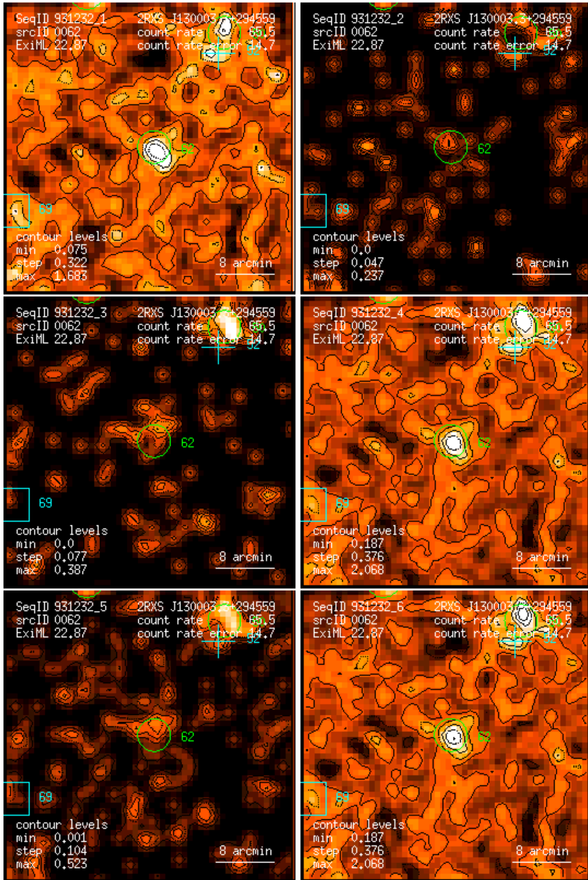
Figure 62: RASS 931232: detection 0062: band rate images, Gaussian filter: (1) PSPC channels 11 – 41, (2) 52 – 90, (3) 91 – 201, (4) 11 – 235, (5) 52 – 201, (6) 11 – 201. Broad band rates in counts/ks. Band rate contour levels in counts/ks/arcmin 2 .
