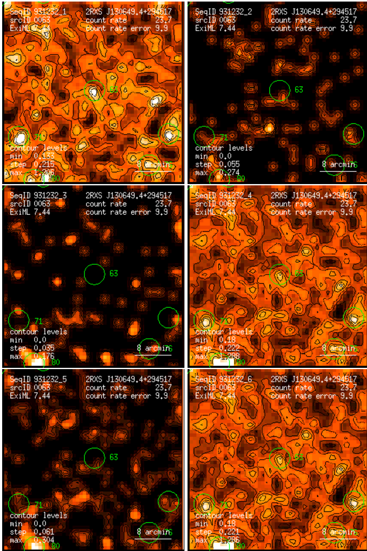
Figure 63: RASS 931232: detection 0063: band rate images, Gaussian filter: (1) PSPC channels 11 – 41, (2) 52 – 90, (3) 91 – 201, (4) 11 – 235, (5) 52 – 201, (6) 11 – 201. Broad band rates in counts/ks. Band rate contour levels in counts/ks/arcmin 2 .
