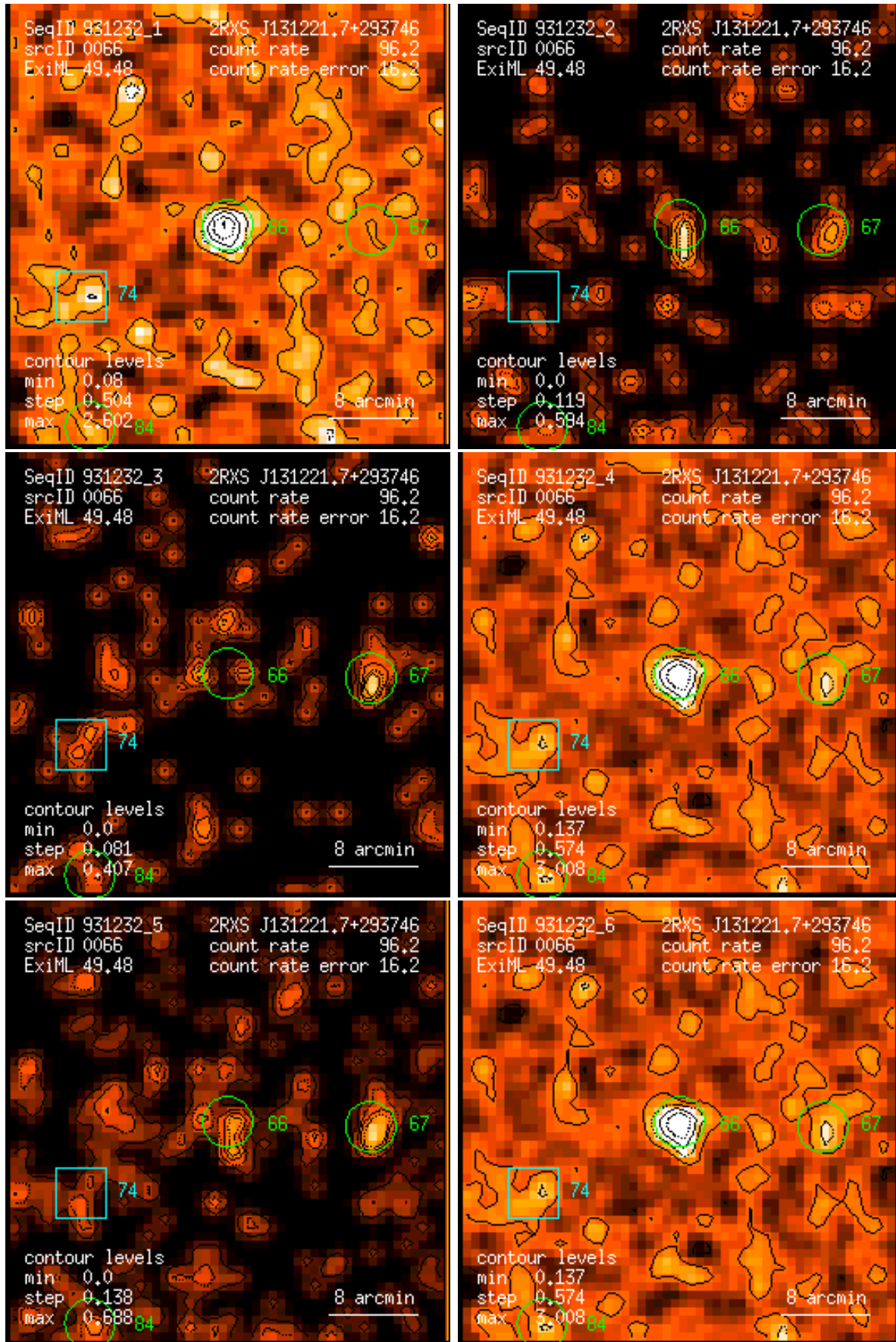
Figure 66: RASS 931232: detection 0066: band rate images, Gaussian filter: (1) PSPC channels 11 – 41, (2) 52 – 90, (3) 91 – 201, (4) 11 – 235, (5) 52 – 201, (6) 11 – 201. Broad band rates in counts/ks. Band rate contour levels in counts/ks/arcmin 2 .
