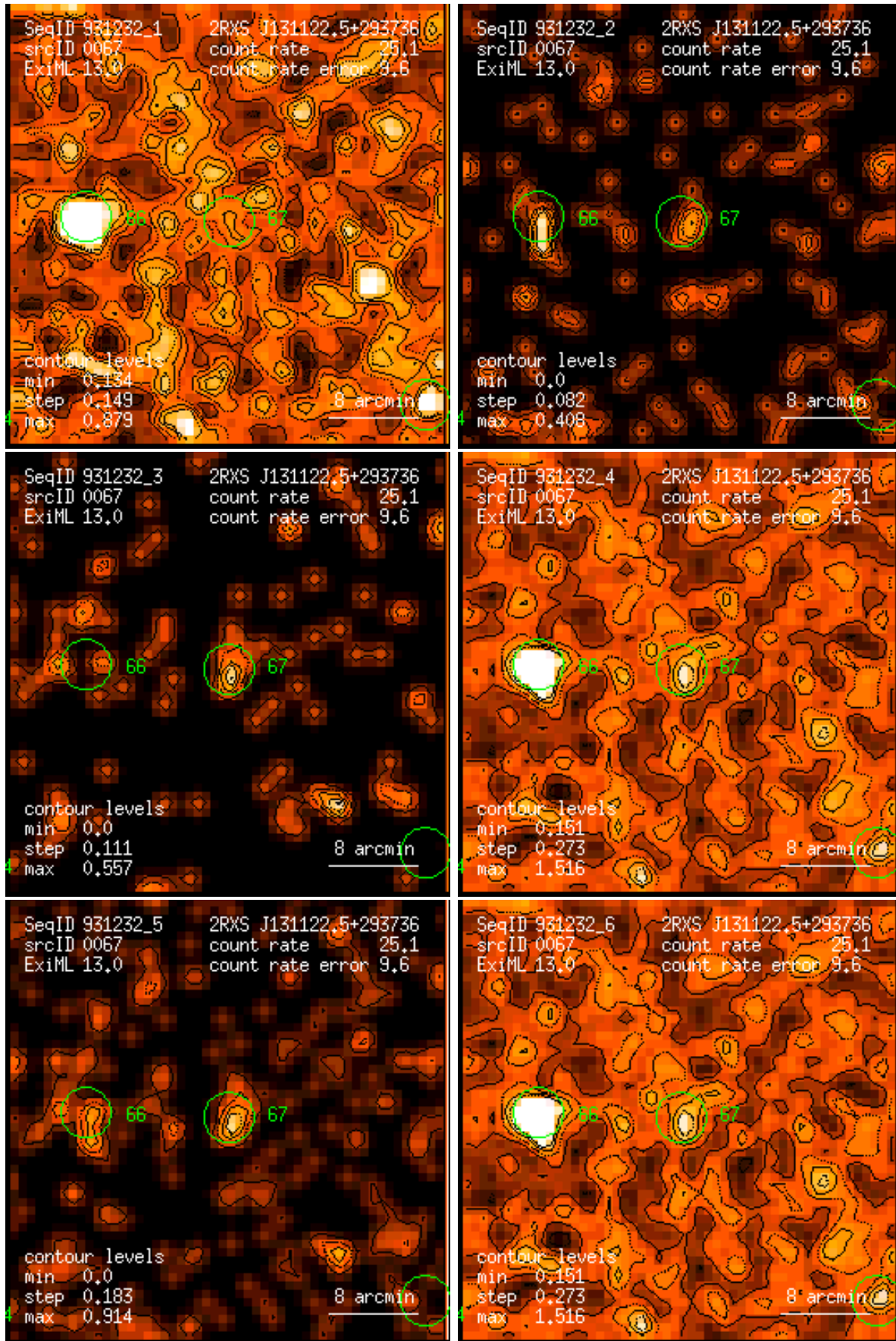
Figure 67: RASS 931232: detection 0067: band rate images, Gaussian filter: (1) PSPC channels 11 – 41, (2) 52 – 90, (3) 91 – 201, (4) 11 – 235, (5) 52 – 201, (6) 11 – 201. Broad band rates in counts/ks. Band rate contour levels in counts/ks/arcmin 2 .
