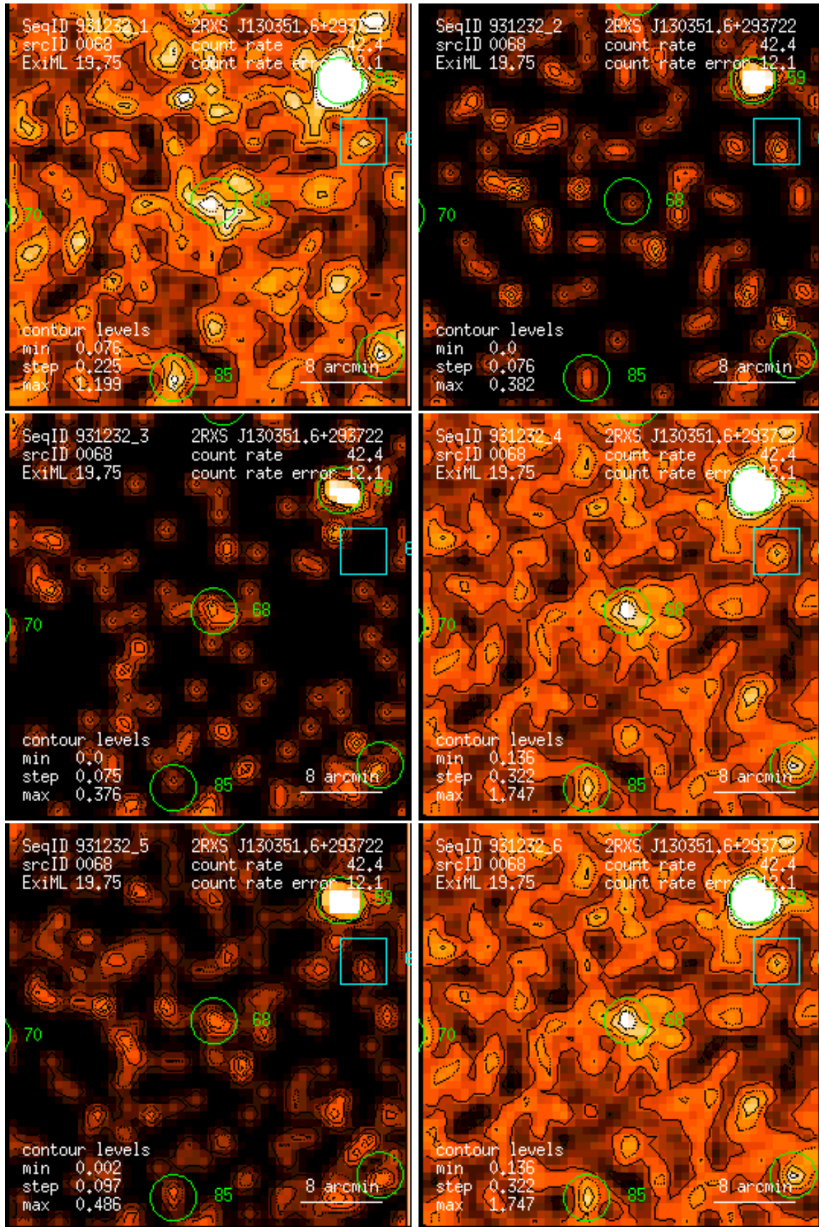
Figure 68: RASS 931232: detection 0068: band rate images, Gaussian filter: (1) PSPC channels 11 – 41, (2) 52 – 90, (3) 91 – 201, (4) 11 – 235, (5) 52 – 201, (6) 11 – 201. Broad band rates in counts/ks. Band rate contour levels in counts/ks/arcmin 2 .
