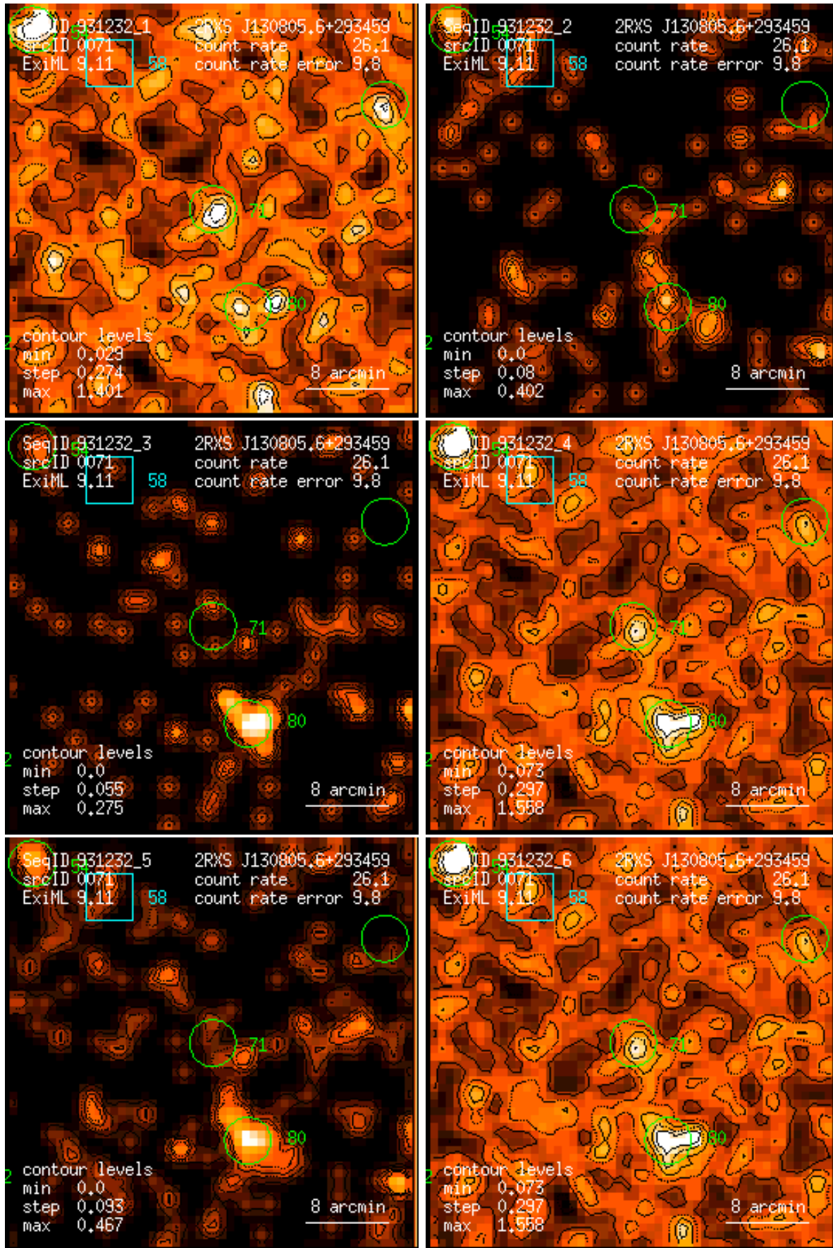
Figure 71: RASS 931232: detection 0071: band rate images, Gaussian filter: (1) PSPC channels 11 – 41, (2) 52 – 90, (3) 91 – 201, (4) 11 – 235, (5) 52 – 201, (6) 11 – 201. Broad band rates in counts/ks. Band rate contour levels in counts/ks/arcmin 2 .
