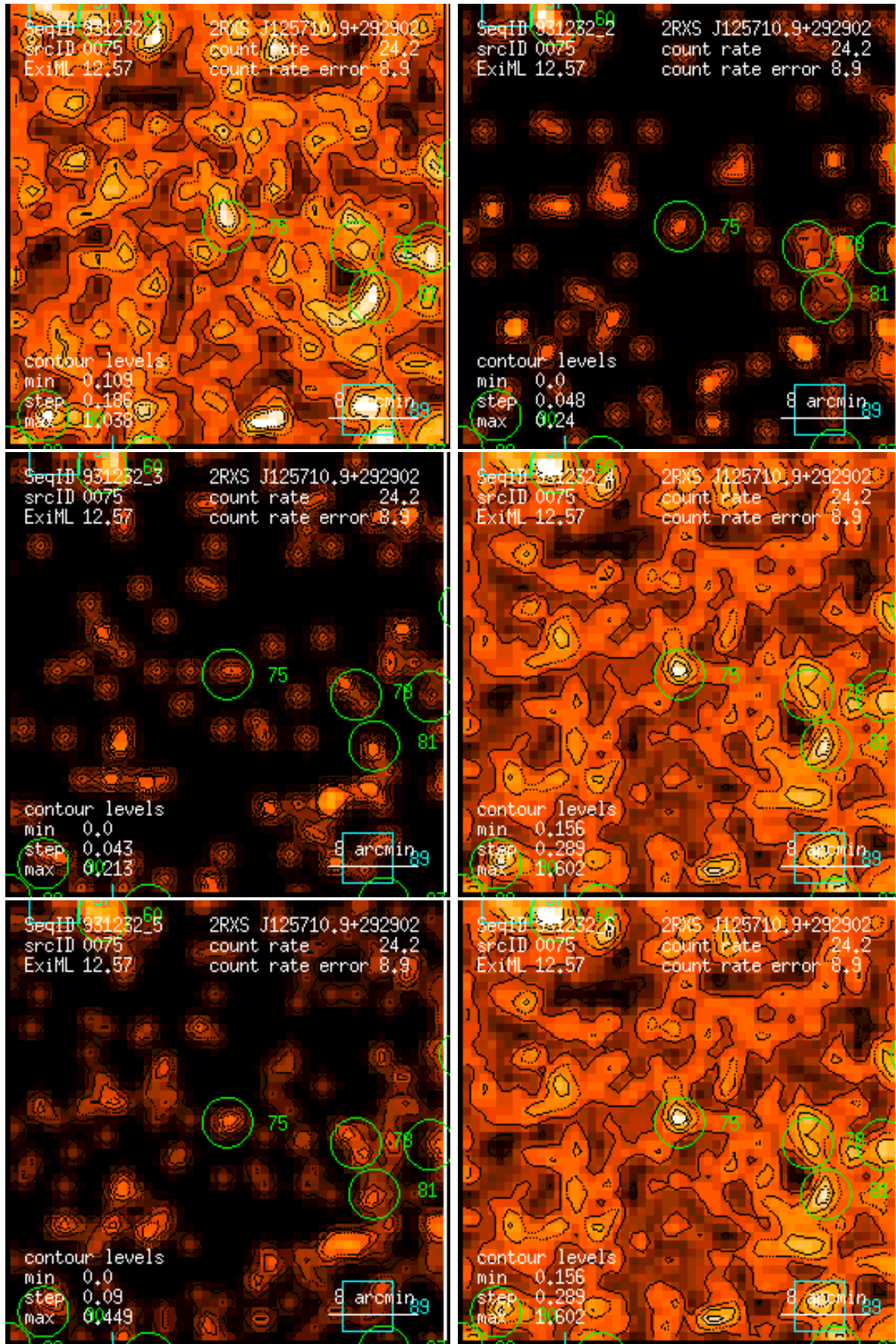
Figure 75: RASS 931232: detection 0075: band rate images, Gaussian filter: (1) PSPC channels 11 – 41, (2) 52 – 90, (3) 91 – 201, (4) 11 – 235, (5) 52 – 201, (6) 11 – 201. Broad band rates in counts/ks. Band rate contour levels in counts/ks/arcmin 2 .
