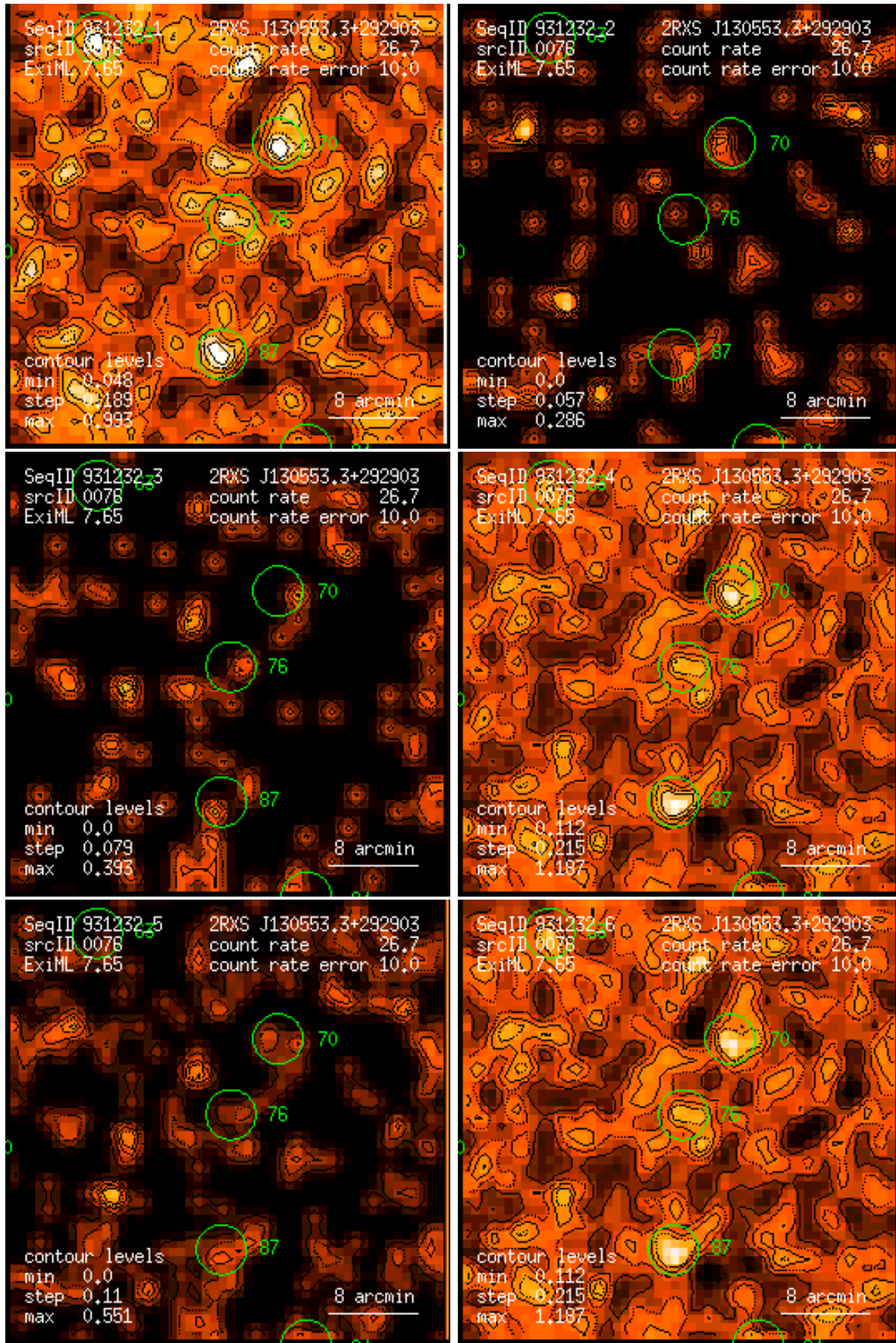
Figure 76: RASS 931232: detection 0076: band rate images, Gaussian filter: (1) PSPC channels 11 – 41, (2) 52 – 90, (3) 91 – 201, (4) 11 – 235, (5) 52 – 201, (6) 11 – 201. Broad band rates in counts/ks. Band rate contour levels in counts/ks/arcmin 2 .
