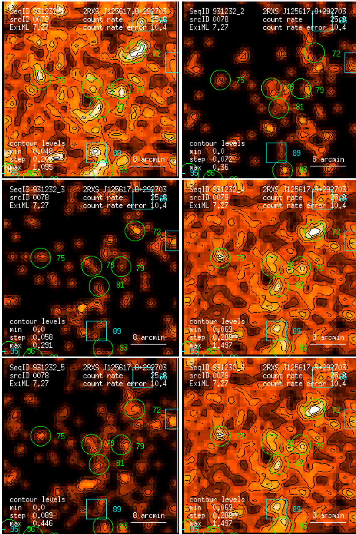
Figure 78: RASS 931232: detection 0078: band rate images, Gaussian filter: (1) PSPC channels 11 – 41, (2) 52 – 90, (3) 91 – 201, (4) 11 – 235, (5) 52 – 201, (6) 11 – 201. Broad band rates in counts/ks. Band rate contour levels in counts/ks/arcmin 2 .
