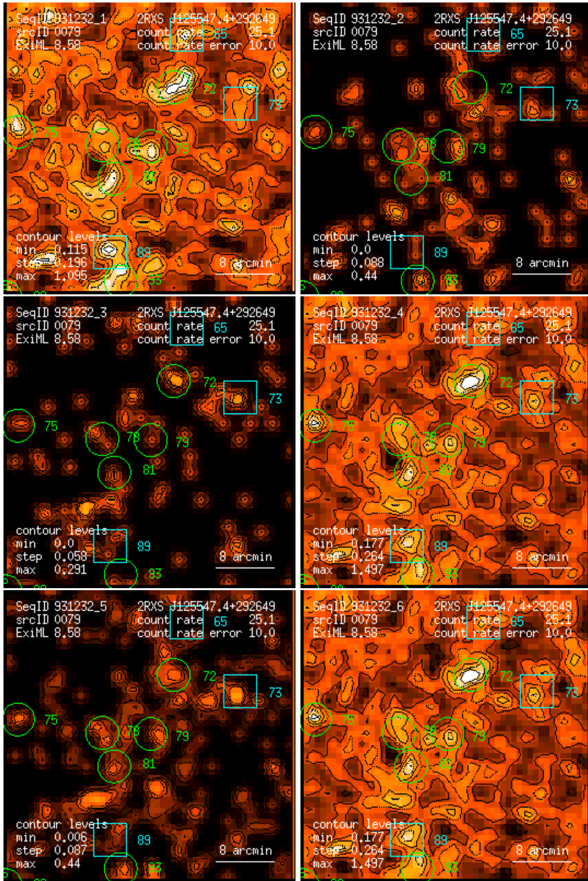
Figure 79: RASS 931232: detection 0079: band rate images, Gaussian filter: (1) PSPC channels 11 – 41, (2) 52 – 90, (3) 91 – 201, (4) 11 – 235, (5) 52 – 201, (6) 11 – 201. Broad band rates in counts/ks. Band rate contour levels in counts/ks/arcmin 2 .
