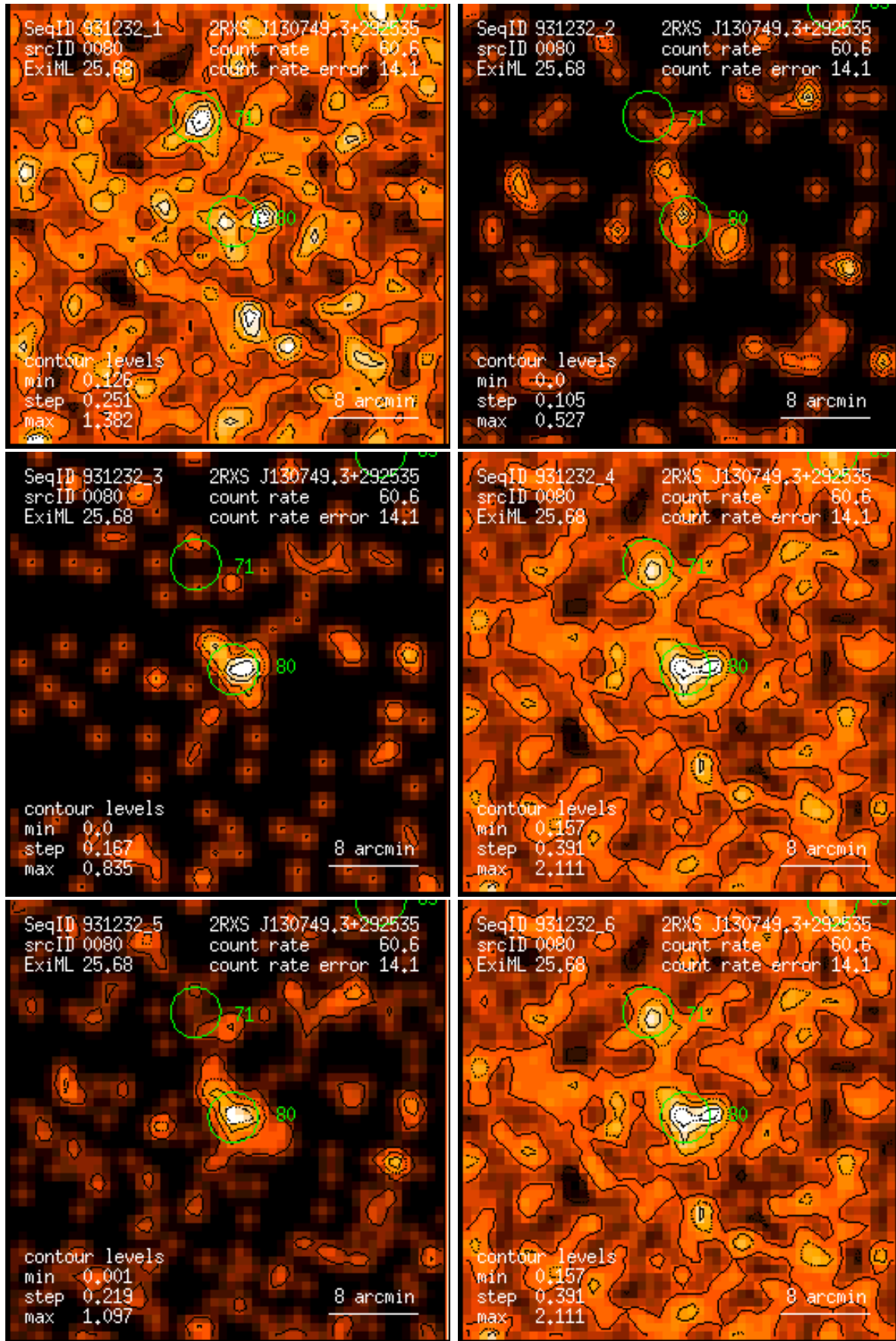
Figure 80: RASS 931232: detection 0080: band rate images, Gaussian filter: (1) PSPC channels 11 – 41, (2) 52 – 90, (3) 91 – 201, (4) 11 – 235, (5) 52 – 201, (6) 11 – 201. Broad band rates in counts/ks. Band rate contour levels in counts/ks/arcmin 2 .
