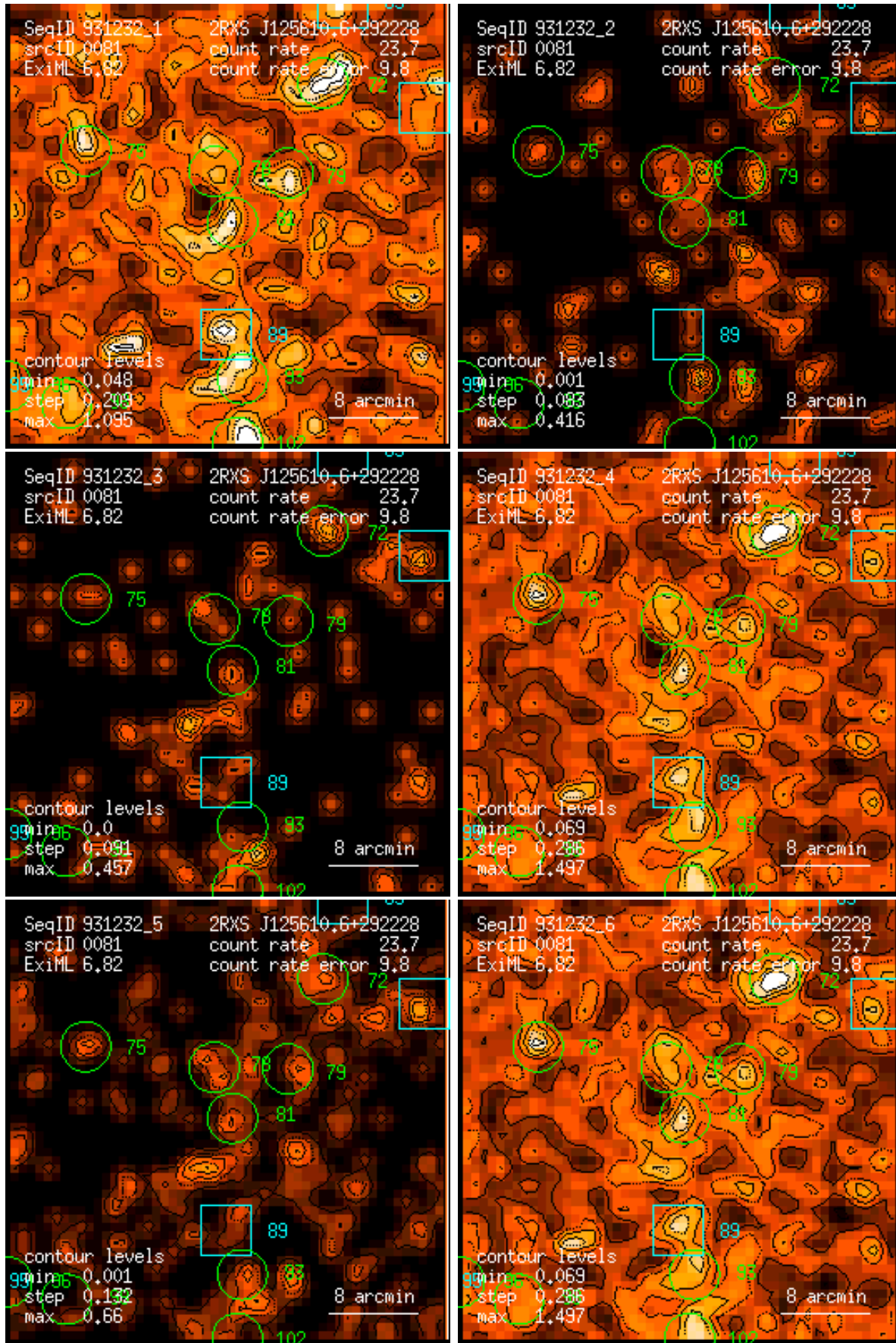
Figure 81: RASS 931232: detection 0081: band rate images, Gaussian filter: (1) PSPC channels 11 – 41, (2) 52 – 90, (3) 91 – 201, (4) 11 – 235, (5) 52 – 201, (6) 11 – 201. Broad band rates in counts/ks. Band rate contour levels in counts/ks/arcmin 2 .
