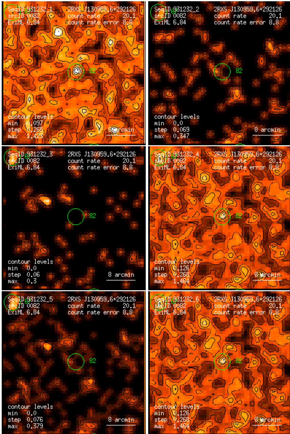
Figure 82: RASS 931232: detection 0082: band rate images, Gaussian filter: (1) PSPC channels 11 – 41, (2) 52 – 90, (3) 91 – 201, (4) 11 – 235, (5) 52 – 201, (6) 11 – 201. Broad band rates in counts/ks. Band rate contour levels in counts/ks/arcmin 2 .
