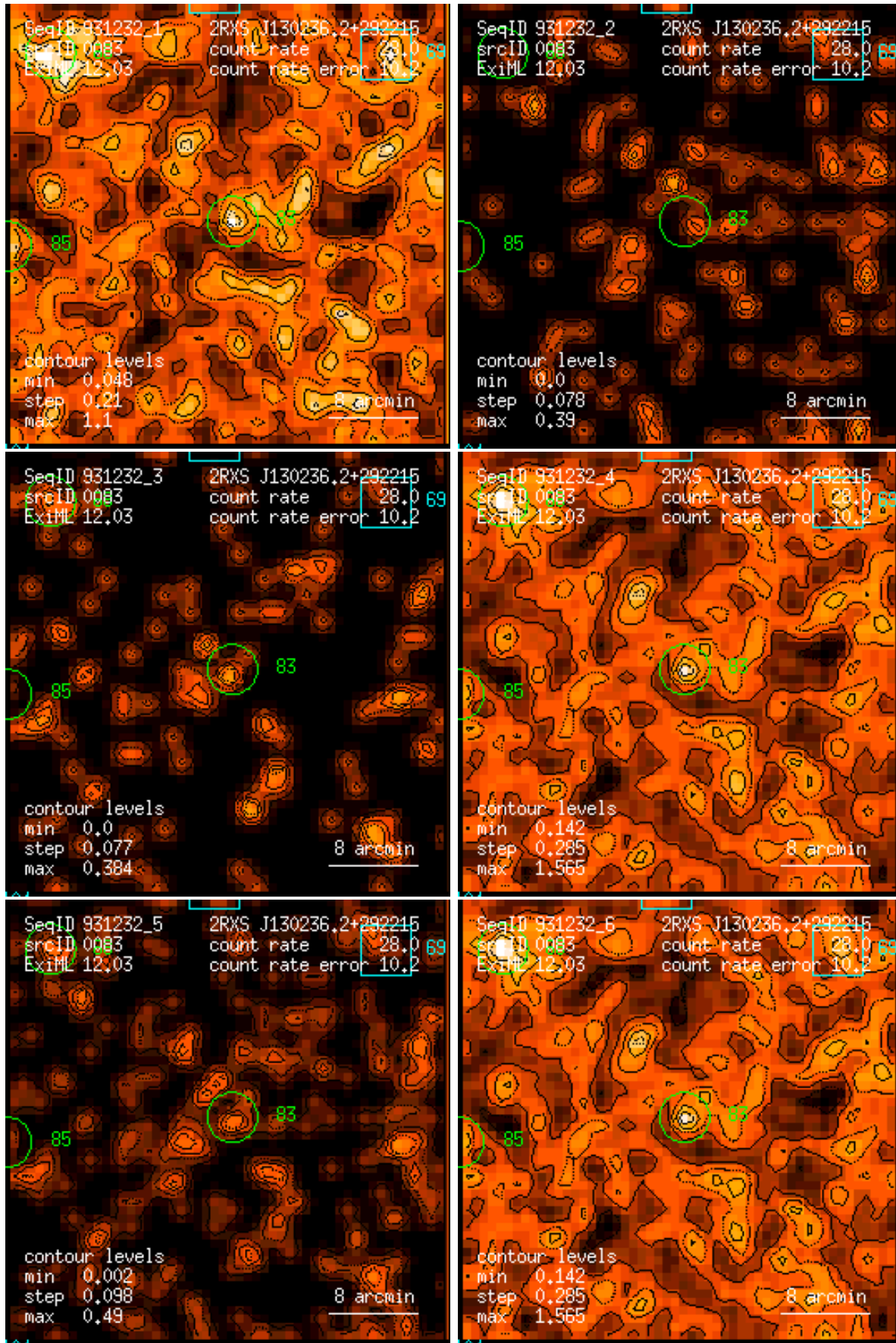
Figure 83: RASS 931232: detection 0083: band rate images, Gaussian filter: (1) PSPC channels 11 – 41, (2) 52 – 90, (3) 91 – 201, (4) 11 – 235, (5) 52 – 201, (6) 11 – 201. Broad band rates in counts/ks. Band rate contour levels in counts/ks/arcmin 2 .
