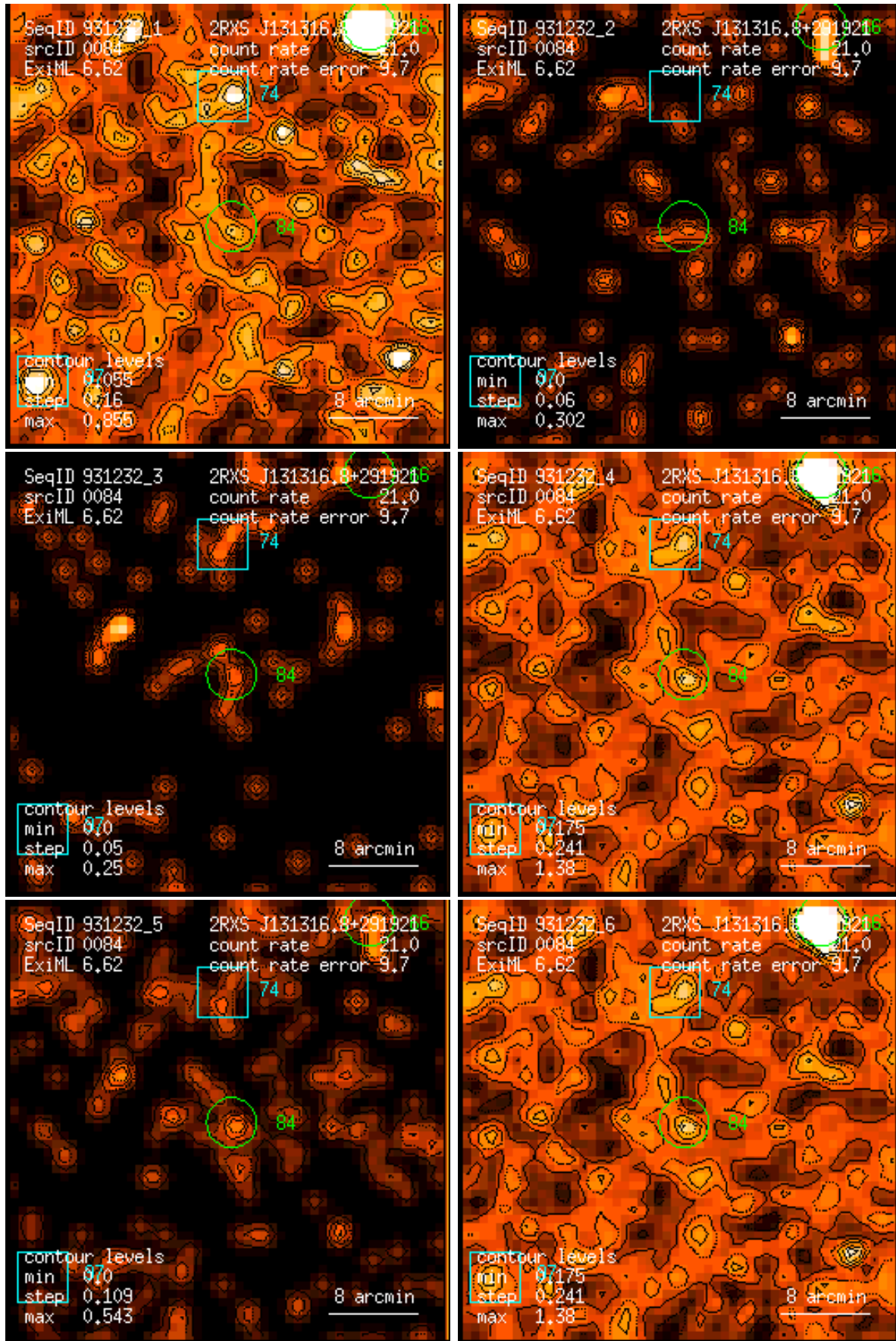
Figure 84: RASS 931232: detection 0084: band rate images, Gaussian filter: (1) PSPC channels 11 – 41, (2) 52 – 90, (3) 91 – 201, (4) 11 – 235, (5) 52 – 201, (6) 11 – 201. Broad band rates in counts/ks. Band rate contour levels in counts/ks/arcmin 2 .
