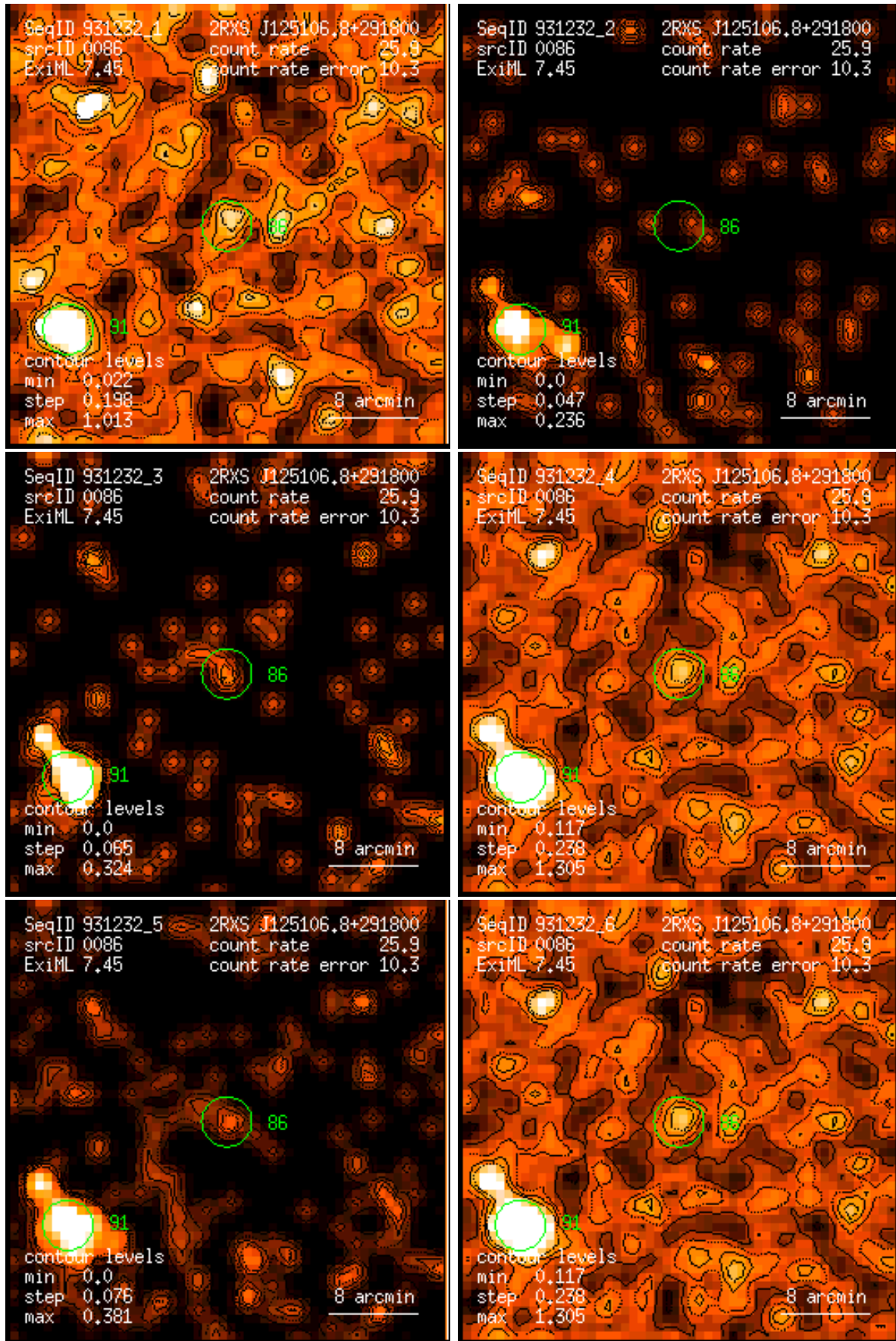
Figure 86: RASS 931232: detection 0086: band rate images, Gaussian filter: (1) PSPC channels 11 – 41, (2) 52 – 90, (3) 91 – 201, (4) 11 – 235, (5) 52 – 201, (6) 11 – 201. Broad band rates in counts/ks. Band rate contour levels in counts/ks/arcmin 2 .
