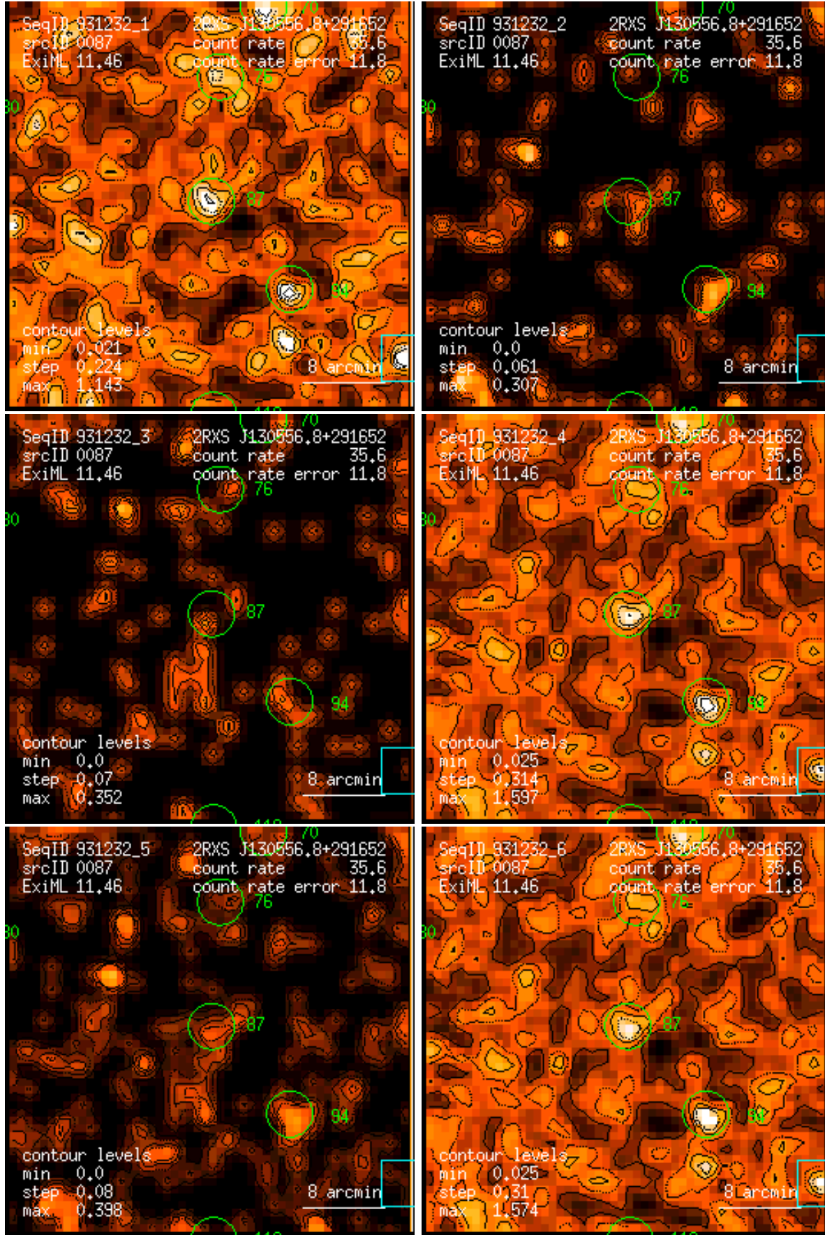
Figure 87: RASS 931232: detection 0087: band rate images, Gaussian filter: (1) PSPC channels 11 – 41, (2) 52 – 90, (3) 91 – 201, (4) 11 – 235, (5) 52 – 201, (6) 11 – 201. Broad band rates in counts/ks. Band rate contour levels in counts/ks/arcmin 2 .
