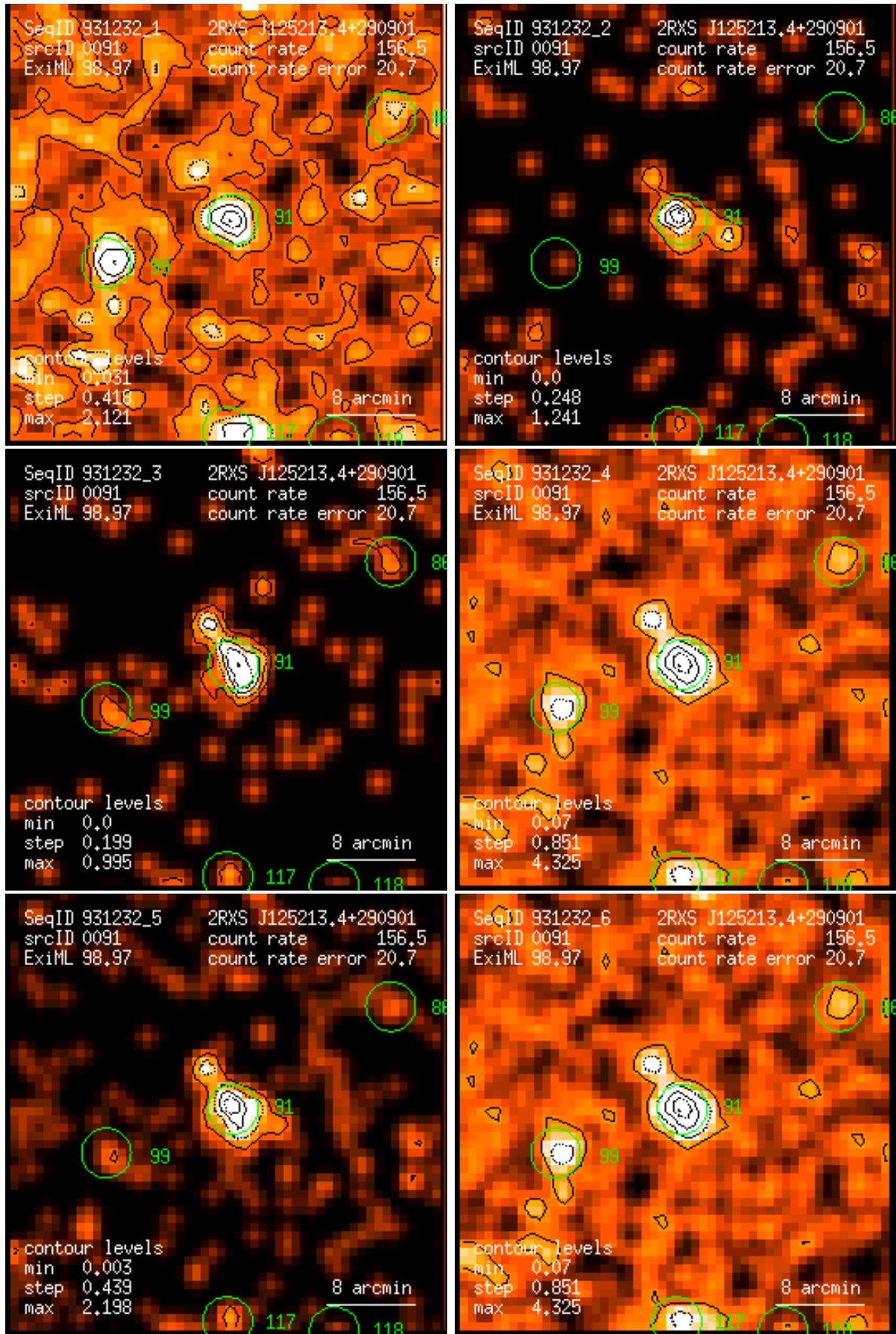
Figure 91: RASS 931232: detection 0091: band rate images, Gaussian filter: (1) PSPC channels 11 – 41, (2) 52 – 90, (3) 91 – 201, (4) 11 – 235, (5) 52 – 201, (6) 11 – 201. Broad band rates in counts/ks. Band rate contour levels in counts/ks/arcmin 2 .
